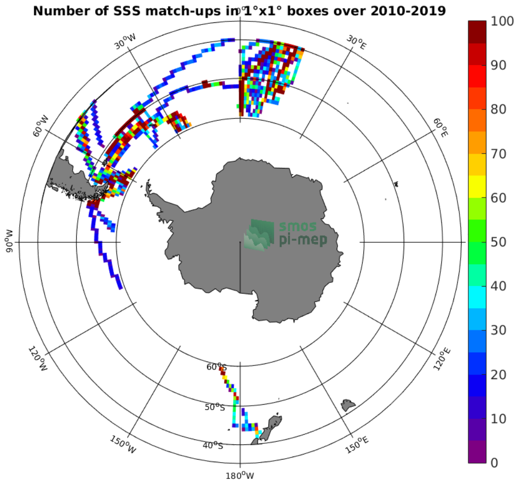
Figure 4: Number of SSS match-ups between TSG-POLARSTERN SSS and the SMOS-L3-CATDS-CECOS-LOCEAN-V4-9DAYS-25KM SSS product for the Roaring Forties and Furious Fifties Pi-MEP region over 1°x1° boxes and for the full satellite product period.
