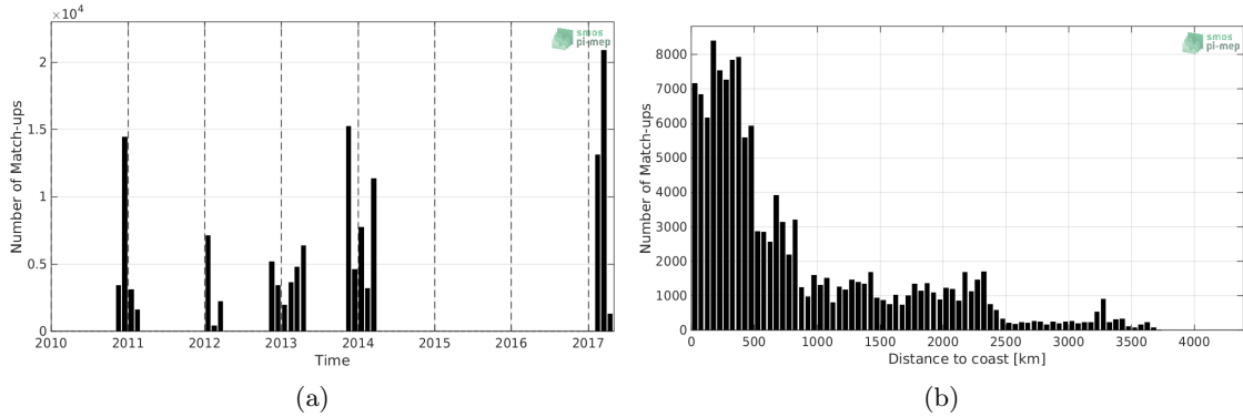
Figure 1: Number of match-ups between TSG-GOSUD-Sailing-ship and SMOS-L3-CATDS-CECOS-LOCEAN-V4-9DAYS-25KM SSS as a function of time (a) and as function of the distance to coast (b) over the Roaring Forties and Furious Fifties Pi-MEP region and for the full satellite product period.
