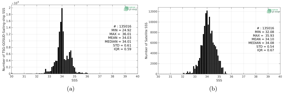
Figure 2: Histograms of SSS from TSG-GOSUD-Sailing-ship (a) and SMOS-L3-CATDS-CECOS-LOCEAN-V4-9DAYS-25KM (b) considering all match-up pairs per bins of 0.1 over the Roaring Forties and Furious Fifties Pi-MEP region and for the full satellite product period.
