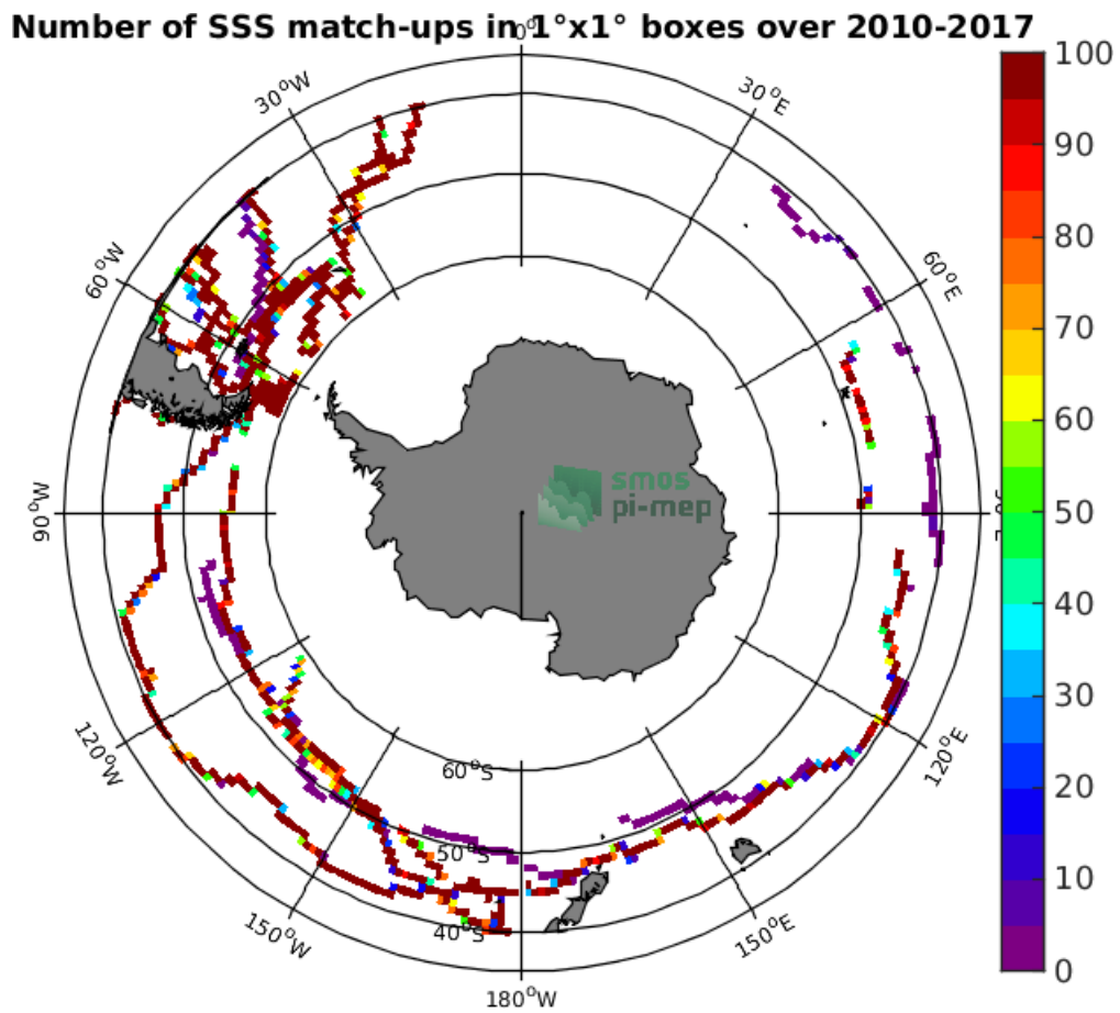
Figure 4: Number of SSS match-ups between TSG-GOSUD-Sailing-ship SSS and the SMOS-L3-CATDS-CECOS-LOCEAN-V4-9DAYS-25KM SSS product for the Roaring Forties and Furious Fifties Pi-MEP region over 1°x1° boxes and for the full satellite product period.
