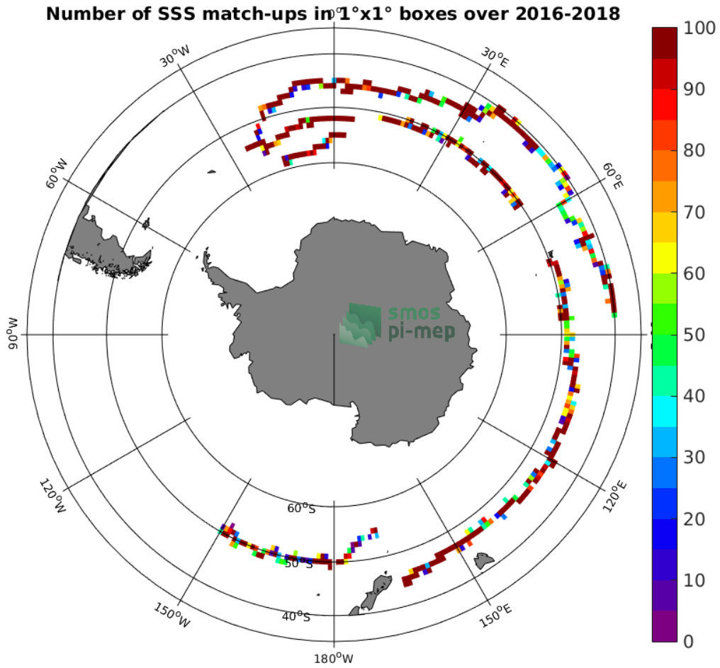
Figure 3: Number of SSS match-ups between Surface drifters SSS and the SMOS-L3-CATDS-CECOS-LOCEAN-V4-9DAYS-25KM SSS product for the Roaring Forties and Furious Fifties Pi-MEP region over 1°x1° boxes and for the full satellite product period.
