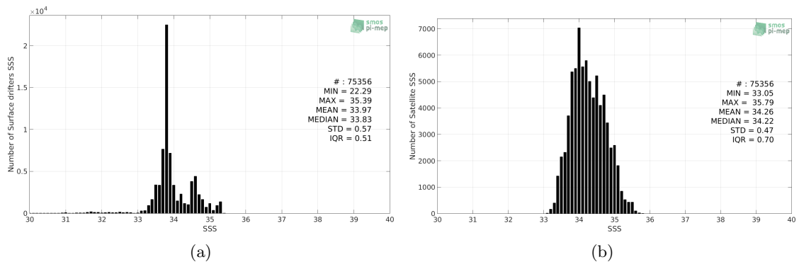
Figure 2: Histograms of SSS from Surface drifters (a) and SMOS-L3-CATDS-CECOS-LOCEAN-V4-9DAYS-25KM (b) considering all match-up pairs per bins of 0.1 over the Roaring Forties and Furious Fifties Pi-MEP region and for the full satellite product period.
