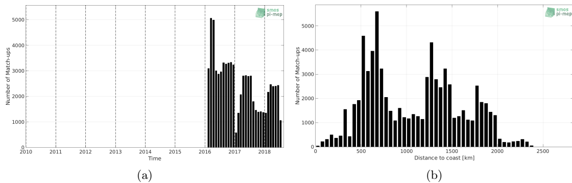
Figure 1: Number of match-ups between Surface drifters and SMOS-L3-CATDS-CECOS-LOCEAN-V4-9DAYS-25KM SSS as a function of time (a) and as function of the distance to coast (b) over the Roaring Forties and Furious Fifties Pi-MEP region and for the full satellite product period.
