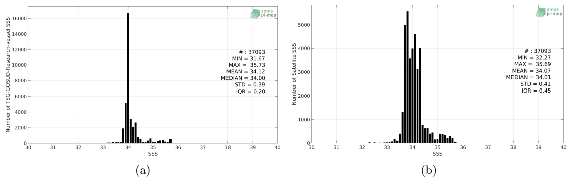
Figure 2: Histograms of SSS from TSG-GOSUD-Research-vessel (a) and SMOS-L3-CATDS-CECOS-LOCEAN-V4-18DAYS-25KM (b) considering all match-up pairs per bins of 0.1 over the Roaring Forties and Furious Fifties Pi-MEP region and for the full satellite product period.
