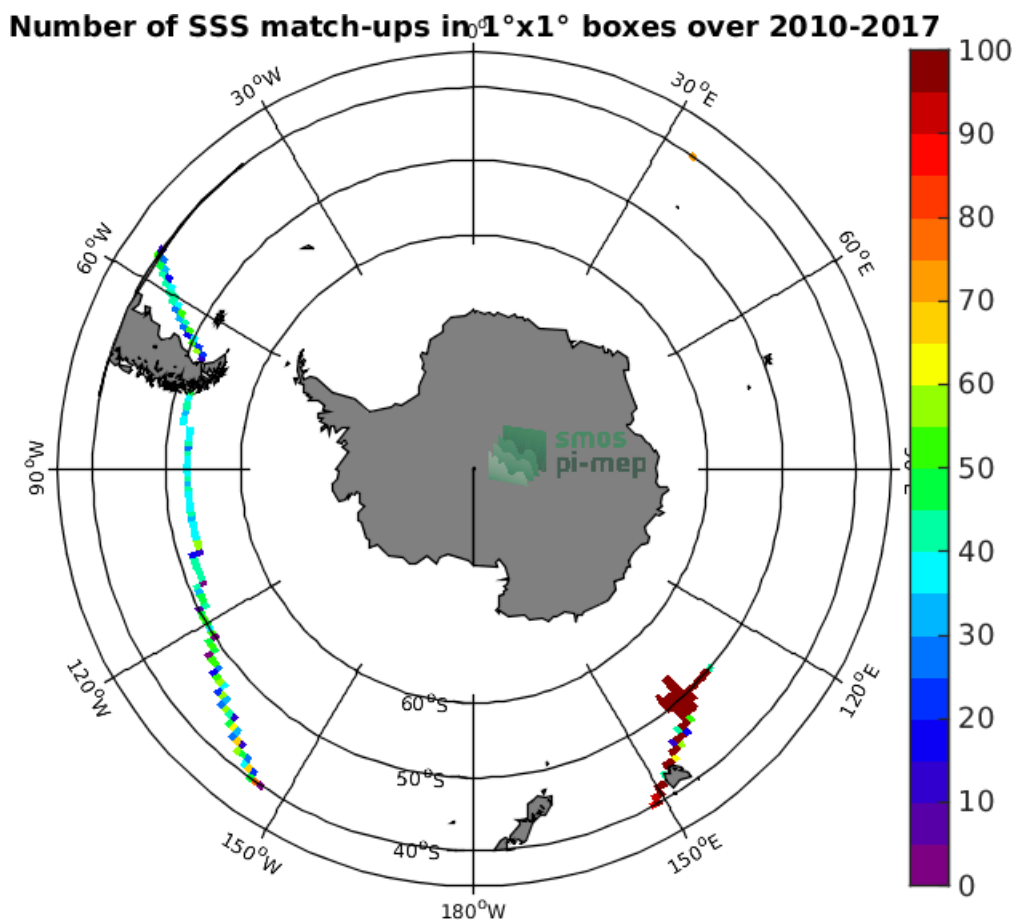
Figure 4: Number of SSS match-ups between TSG-GOSUD-Research-vessel SSS and the SMOS-L3-CATDS-CECOS-LOCEAN-V4-18DAYS-25KM SSS product for the Roaring Forties and Furious Fifties Pi-MEP region over 1°x1° boxes and for the full satellite product period.
