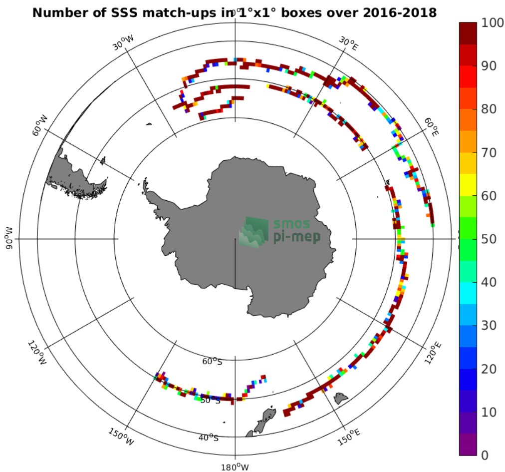
Figure 3: Number of SSS match-ups between Surface drifters SSS and the SMOS-L3-CATDS-CECOS-LOCEAN-V4-18DAYS-25KM SSS product for the Roaring Forties and Furious Fifties Pi-MEP region over 1^\circ \times 1^\circ boxes and for the full satellite product period.
