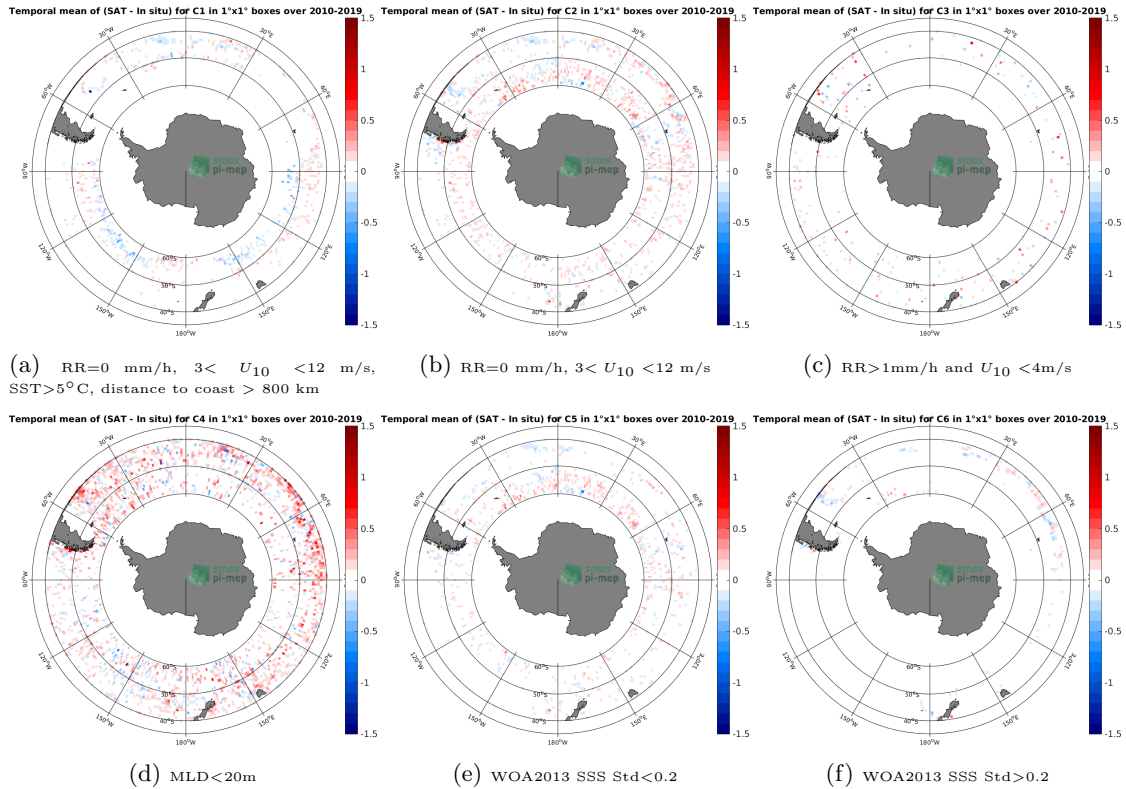
Figure 12: Temporal mean gridded over spatial boxes of size 1^{\circ}\times 1^{\circ} of \Delta\text{SSS} (SMOS-L3-CATDS-CECOS-LOCEAN-V4-18DAYS-25KM - Argo) for 6 different subdatasets corresponding to:RR=0 mm/h, 3 < U_{10} < 12 m/s, SST >5^{\circ}\text{C} , distance to coast > 800 km (a), RR=0 mm/h, 3 < U_{10} < 12 m/s (b), RR >1\text{mm/h} and U_{10} < 4\text{m/s} (c),MLD <20\text{m} (d),WOA2013 SSS Std <0.2 (e),WOA2013 SSS Std >0.2 (f).
