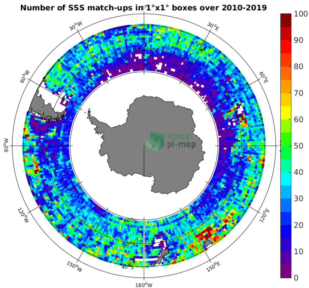
Figure 4: Number of SSS match-ups between Argo SSS and the SMOS-L3-CATDS-CECOS-LOCEAN-V4-18DAYS-25KM SSS product for the Roaring Forties and Furious Fifties Pi-MEP region over 1^\circ \times 1^\circ boxes and for the full satellite product period.
