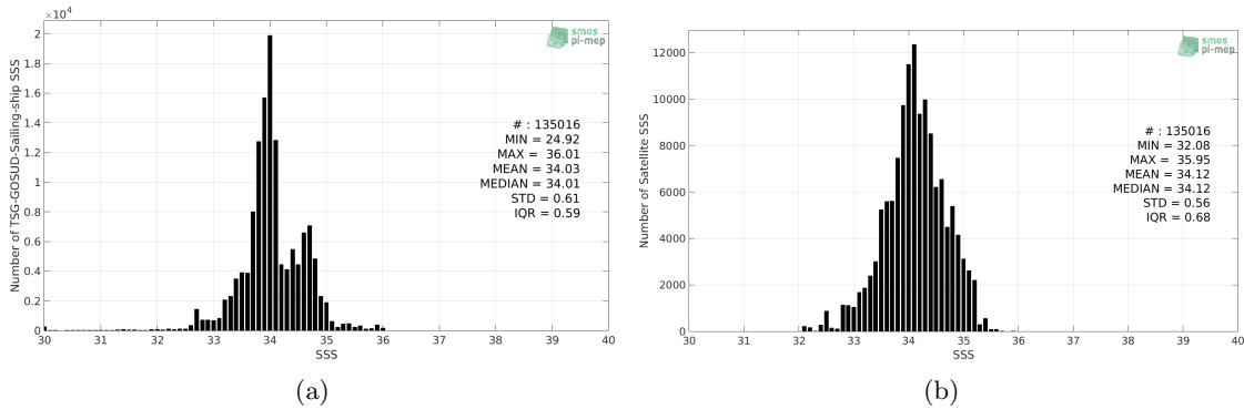
Figure 2: Histograms of SSS from TSG-GOSUD-Sailing-ship (a) and SMOS-L3-CATDS-CECOS-LOCEAN-V3-9DAYS-25KM (b) considering all match-up pairs per bins of 0.1 over the Roaring Forties and Furious Fifties Pi-MEP region and for the full satellite product period.
