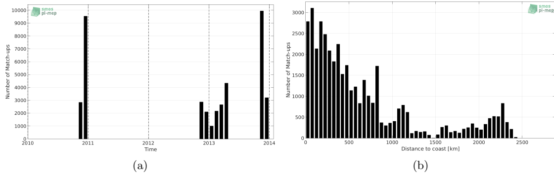
Figure 1: Number of match-ups between TSG-GOSUD-Sailing-ship and SMOS-L3-CATDS-CECOS-LOCEAN-V3-9DAYS-25KM SSS as a function of time (a) and as function of the distance to coast (b) over the Roaring Forties and Furious Fifties Pi-MEP region and for the full satellite product period.
