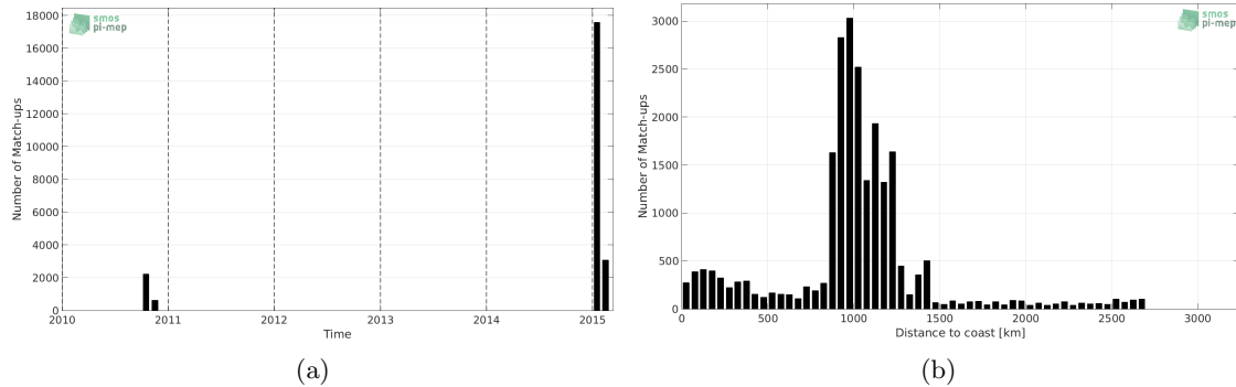
Figure 1: Number of match-ups between TSG-GOSUD-Research-vessel and SMOS-L3-CATDS-CECOS-LOCEAN-V3-9DAYS-25KM SSS as a function of time (a) and as function of the distance to coast (b) over the Roaring Forties and Furious Fifties Pi-MEP region and for the full satellite product period.
