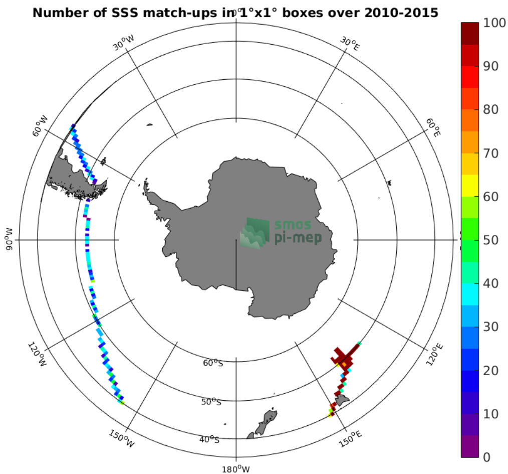
Figure 4: Number of SSS match-ups between TSG-GOSUD-Research-vessel SSS and the SMOS-L3-CATDS-CECOS-LOCEAN-V3-9DAYS-25KM SSS product for the Roaring Forties and Furious Fifties Pi-MEP region over 1^\circ \times 1^\circ boxes and for the full satellite product period.
