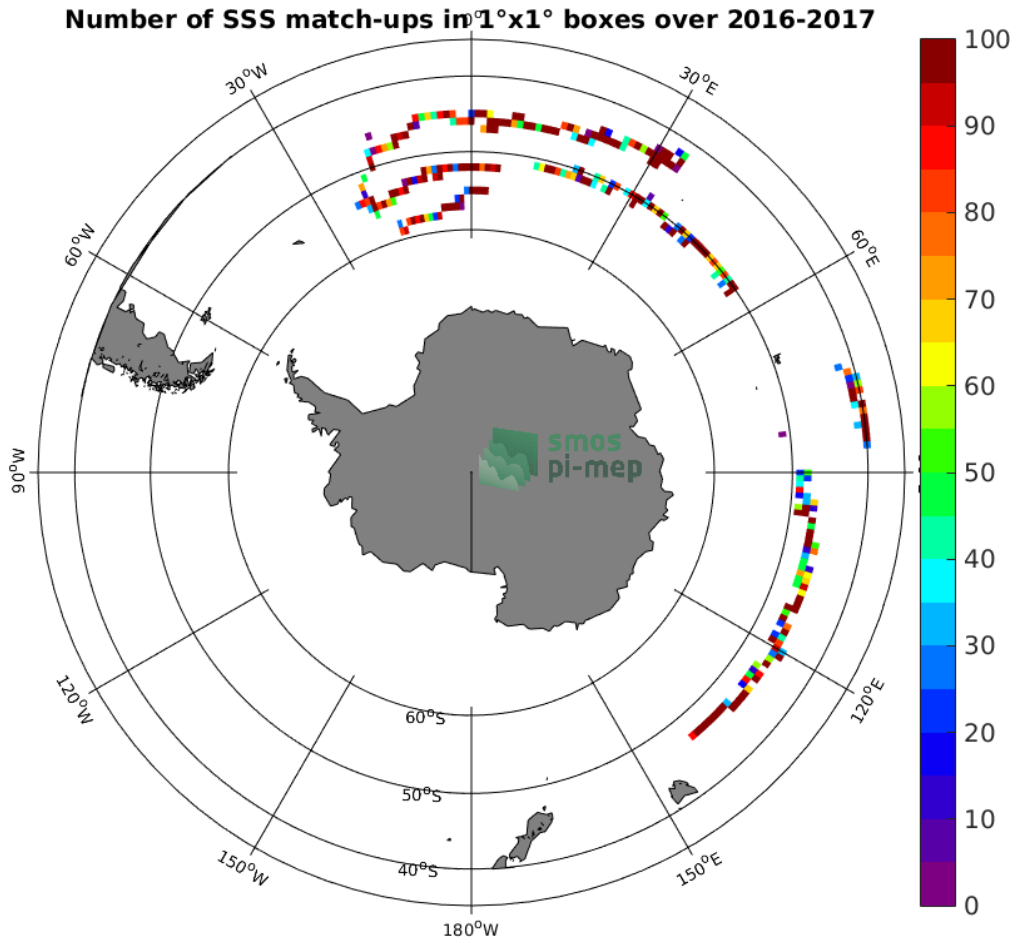
Figure 3: Number of SSS match-ups between Surface drifters SSS and the SMOS-L3-CATDS-CECOS-LOCEAN-V3-9DAYS-25KM SSS product for the Roaring Forties and Furious Fifties Pi-MEP region over 1°x1° boxes and for the full satellite product period.
