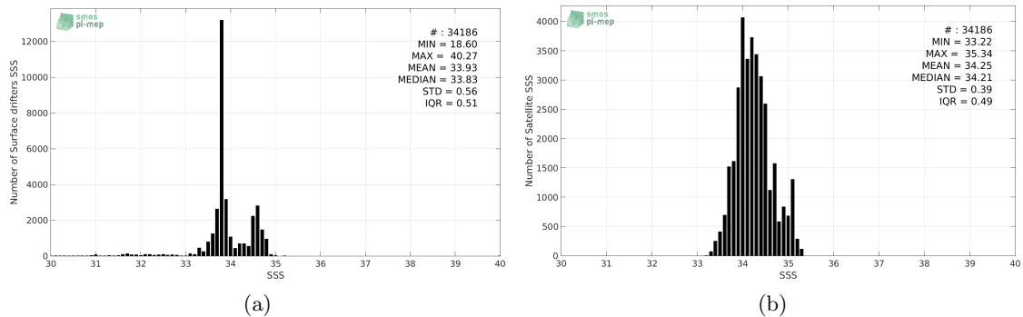
Figure 2: Histograms of SSS from Surface drifters (a) and SMOS-L3-CATDS-CECOS-LOCEAN-V3-9DAYS-25KM (b) considering all match-up pairs per bins of 0.1 over the Roaring Forties and Furious Fifties Pi-MEP region and for the full satellite product period.
