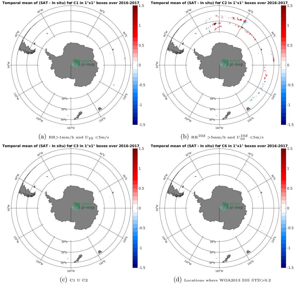
Figure 11: Temporal mean gridded over spatial boxes of size 1^\circ \times 1^\circ of \Delta SSS (SMOS-L3-CATDS-CECOS-LOCEAN-V3-9DAYS-25KM - Surface drifters) for 4 different subdatasets corresponding to: RR > 1\text{mm/h} and U_{10} < 5\text{m/s} (a), RR^{10d} > 5\text{mm/h} and U_{10}^{10d} < 5\text{m/s} (b), C1 U C2 (c), Locations where WOA2013 SSS STD > 0.2 (d).
