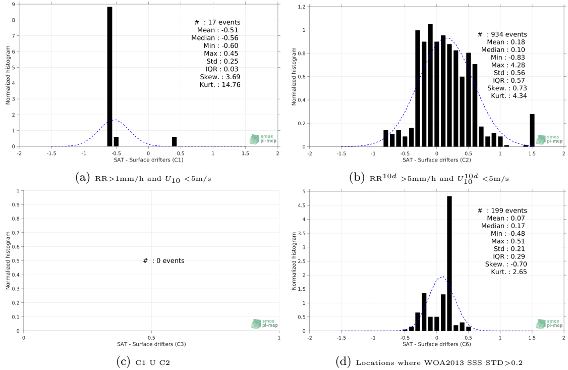
Figure 12: Normalized histogram of \Delta\text{SSS} (SMOS-L3-CATDS-CECOS-LOCEAN-V3-9DAYS-25KM - Surface drifters) for 6 different subdatasets corresponding to: RR > 1\text{mm/h} and U_{10} < 5\text{m/s} (a), RR^{10d} > 5\text{mm/h} and U_{10}^{10d} < 5\text{m/s} (b), C1 U C2 (c), Locations where WOA2013 SSS STD > 0.2 (d).
