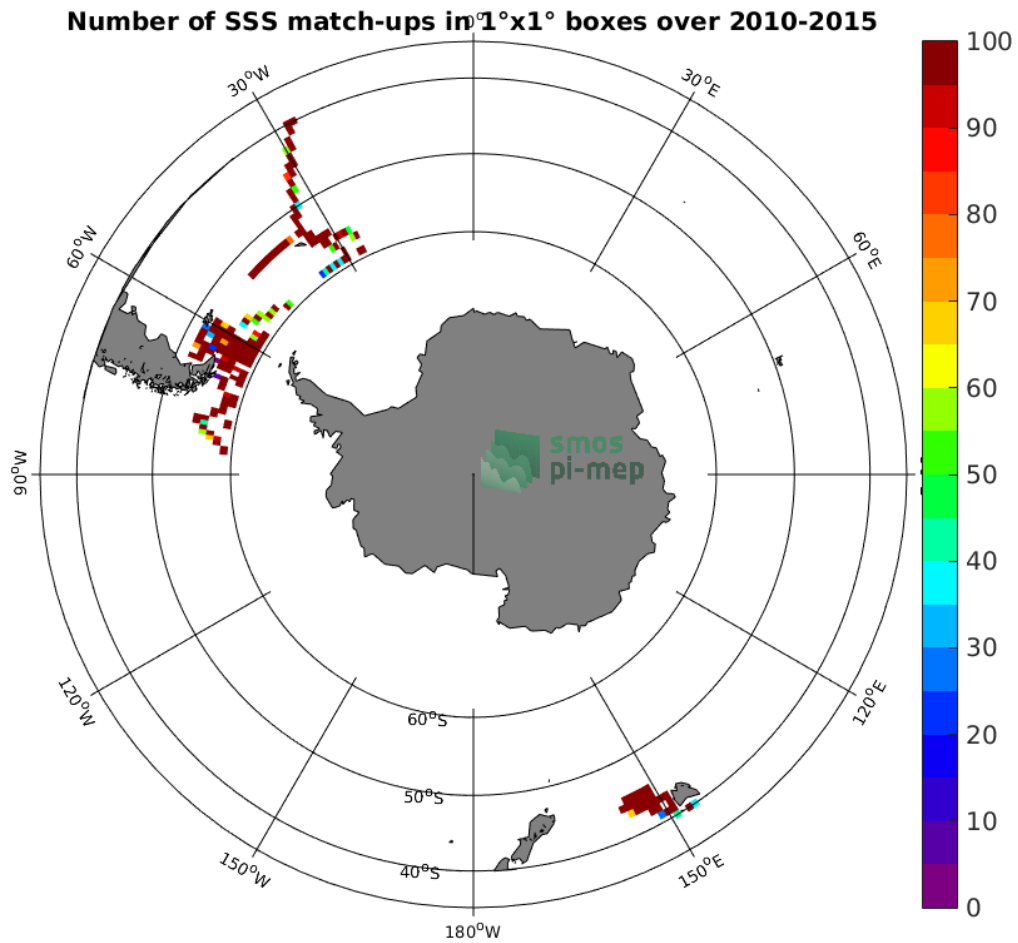
Figure 4: Number of SSS match-ups between TSG-SAMOS SSS and the SMOS-L3-CATDS-CECOS-LOCEAN-V3-18DAYS-25KM SSS product for the Roaring Forties and Furious Fifties Pi-MEP region over 1^\circ \times 1^\circ boxes and for the full satellite product period.
