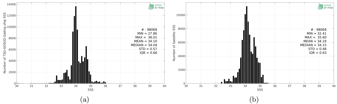
Figure 2: Histograms of SSS from TSG-GOSUD-Sailing-ship (a) and SMOS-L3-CATDS-CECOS-LOCEAN-V3-18DAYS-25KM (b) considering all match-up pairs per bins of 0.1 over the Roaring Forties and Furious Fifties Pi-MEP region and for the full satellite product period.
