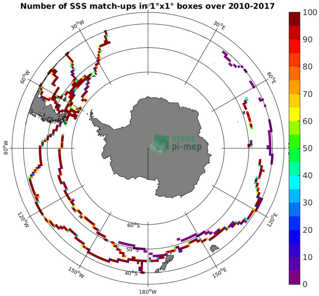
Figure 4: Number of SSS match-ups between TSG-GOSUD-Sailing-ship SSS and the SMOS-L3-CATDS-CECOS-LOCEAN-V3-18DAYS-25KM SSS product for the Roaring Forties and Furious Fifties Pi-MEP region over 1°x1° boxes and for the full satellite product period.
