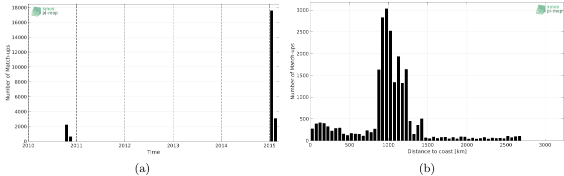
Figure 1: Number of match-ups between TSG-GOSUD-Research-vessel and SMOS-L3-CATDS-CECOS-LOCEAN-V3-18DAYS-25KM SSS as a function of time (a) and as function of the distance to coast (b) over the Roaring Forties and Furious Fifties Pi-MEP region and for the full satellite product period.
