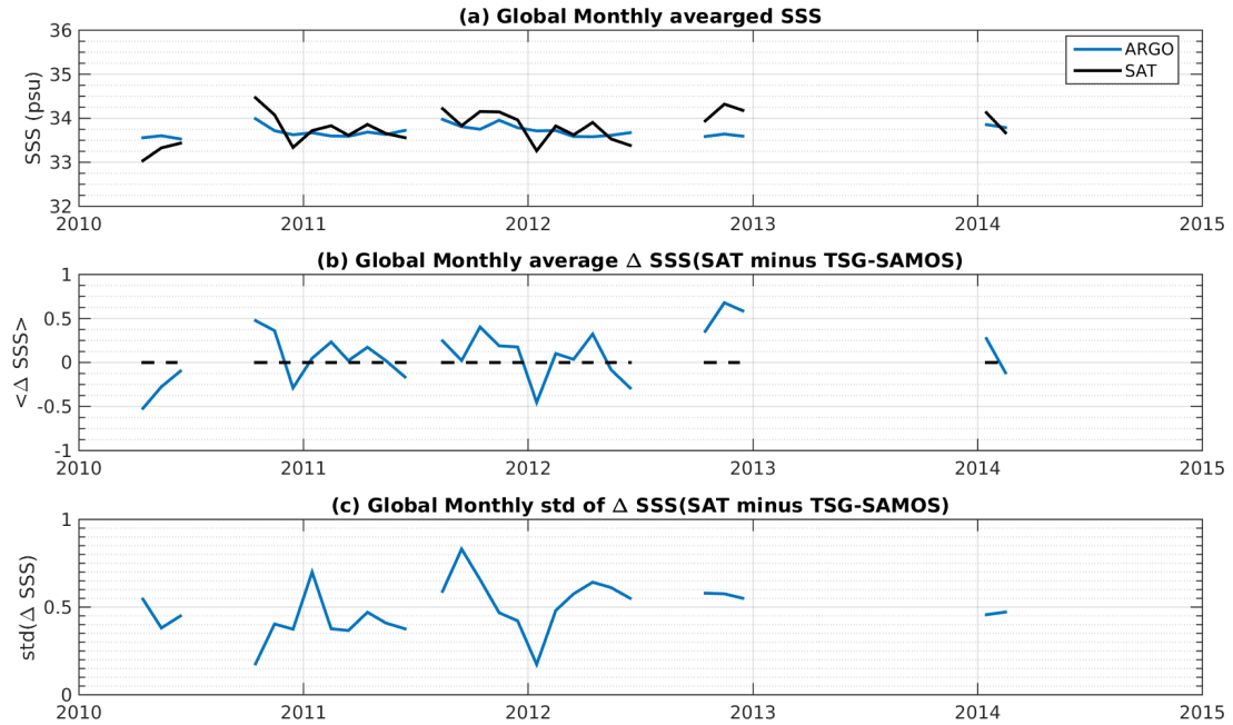
Figure 7: Time series of the monthly averaged mean SSS (top), mean \Delta SSS (Satellite - TSG-SAMOS) and STD of \Delta SSS (Satellite - TSG-SAMOS) over the Roaring Forties and Furious Fifties Pi-MEP region considering all match-ups collected by the Pi-MEP platform.
