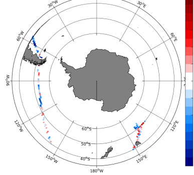
(e) MEAN( \Delta SSS) (Satellite - TSG-GOSUD-Research-vessel)
