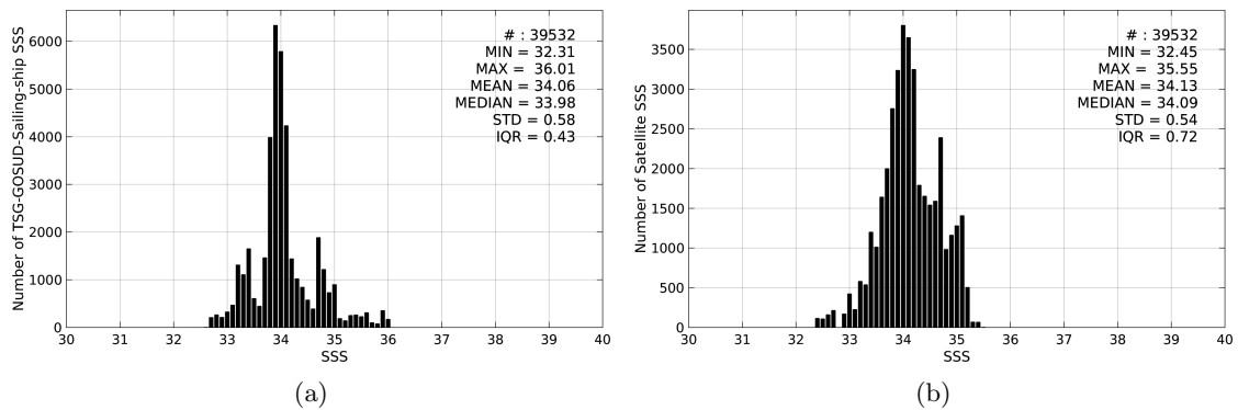
Figure 2: Histograms of SSS from TSG-GOSUD-Sailing-ship (a) and SMOS-L3-CATDS-CECOS-LOCEAN-V2-18DAYS-25KM (b) considering all match-up pairs per bins of 0.1 over the Roaring Forties and Furious Fifties Pi-MEP region and for the full satellite product period.
