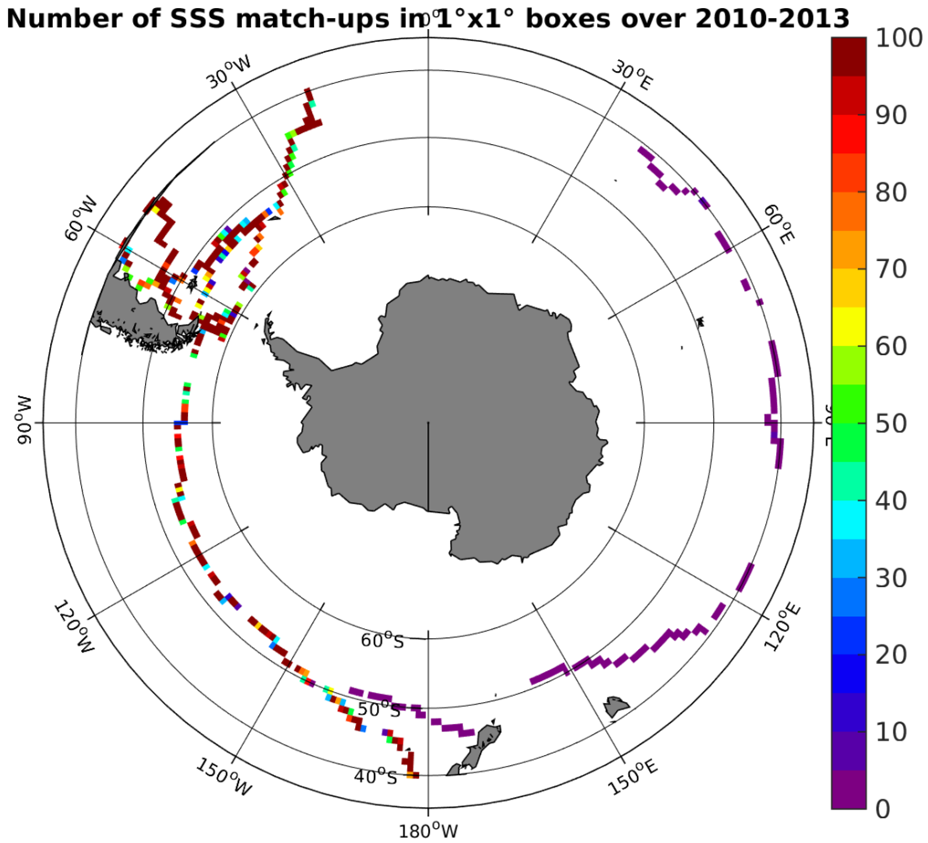
Figure 4: Number of SSS match-ups between TSG-GOSUD-Sailing-ship SSS and the SMOS-L3-CATDS-CECOS-LOCEAN-V2-18DAYS-25KM SSS product for the Roaring Forties and Furious Fifties Pi-MEP region over 1^\circ \times 1^\circ boxes and for the full satellite product period.
