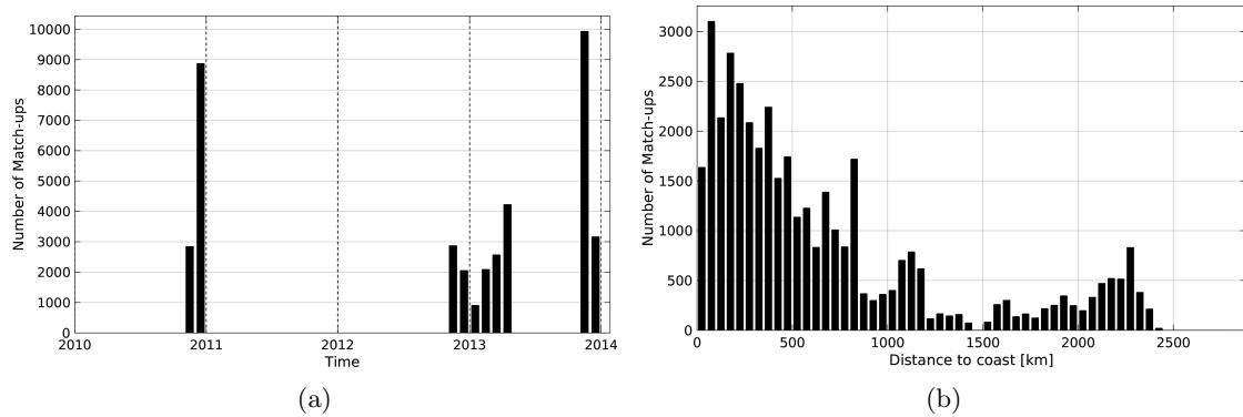
Figure 1: Number of match-ups between TSG-GOSUD-Sailing-ship and SMOS-L3-CATDS-CECOS-LOCEAN-V2-18DAYS-25KM SSS as a function of time (a) and as function of the distance to coast (b) over the Roaring Forties and Furious Fifties Pi-MEP region and for the full satellite product period.
