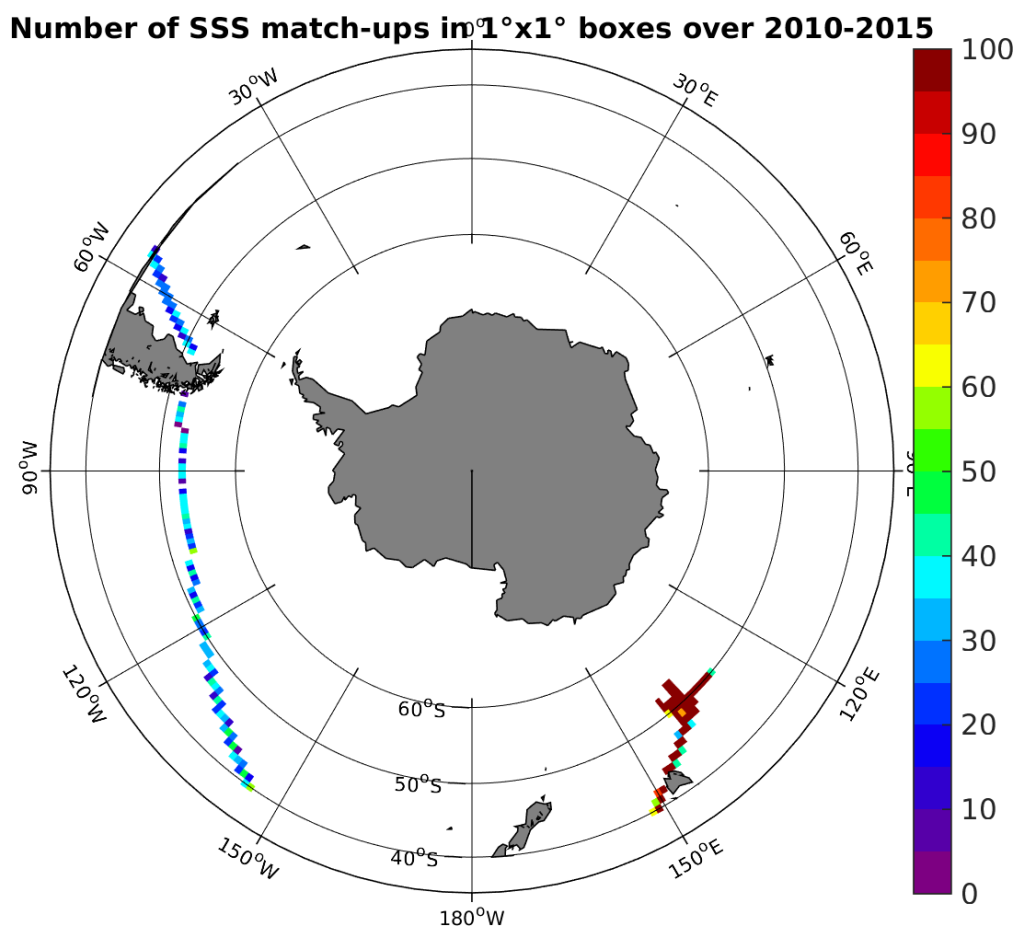
Figure 4: Number of SSS match-ups between TSG-GOSUD-Research-vessel SSS and the SMOS-L3-CATDS-CECOS-LOCEAN-V2-18DAYS-25KM SSS product for the Roaring Forties and Furious Fifties Pi-MEP region over 1^\circ \times 1^\circ boxes and for the full satellite product period.
