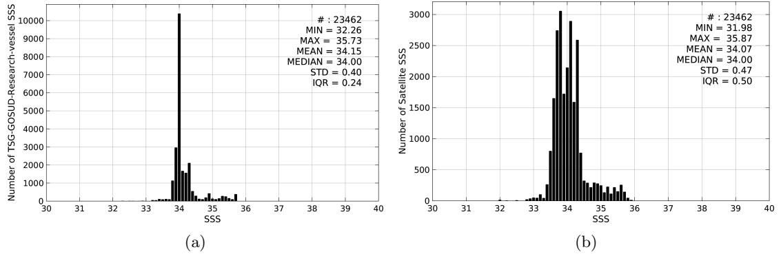
Figure 2: Histograms of SSS from TSG-GOSUD-Research-vessel (a) and SMOS-L3-CATDS-CECOS-LOCEAN-V2-18DAYS-25KM (b) considering all match-up pairs per bins of 0.1 over the Roaring Forties and Furious Fifties Pi-MEP region and for the full satellite product period.
