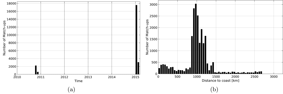
Figure 1: Number of match-ups between TSG-GOSUD-Research-vessel and SMOS-L3-CATDS-CECOS-LOCEAN-V2-18DAYS-25KM SSS as a function of time (a) and as function of the distance to coast (b) over the Roaring Forties and Furious Fifties Pi-MEP region and for the full satellite product period.
