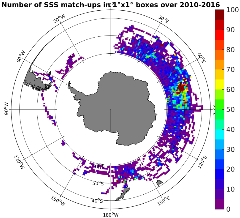
Figure 4: Number of SSS match-ups between Sea mammals SSS and the SMOS-L3-CATDS-CECOS-LOCEAN-V2-18DAYS-25KM SSS product for the Roaring Forties and Furious Fifties Pi-MEP region over 1^\circ \times 1^\circ boxes and for the full satellite product period.
