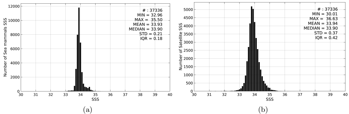
Figure 2: Histograms of SSS from Sea mammals (a) and SMOS-L3-CATDS-CECOS-LOCEAN-V2-18DAYS-25KM (b) considering all match-up pairs per bins of 0.1 over the Roaring Forties and Furious Fifties Pi-MEP region and for the full satellite product period.
