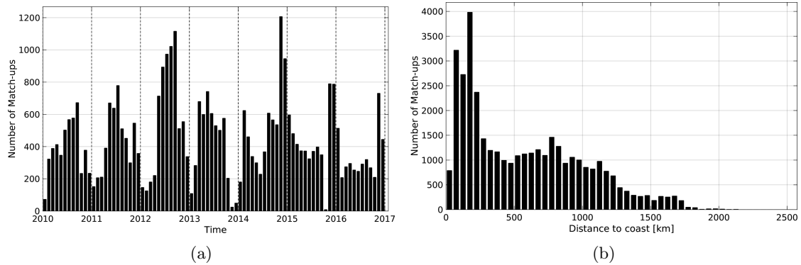
Figure 1: Number of match-ups between Sea mammals and SMOS-L3-CATDS-CECOS-LOCEAN-V2-18DAYS-25KM SSS as a function of time (a) and as function of the distance to coast (b) over the Roaring Forties and Furious Fifties Pi-MEP region and for the full satellite product period.
