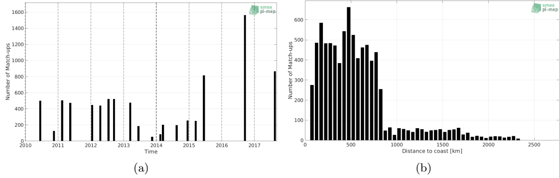
Figure 1: Number of match-ups between TSG (LEGOS-DM) and SMOS SSS L3 v2 - Monthly - 0.25 Deg (CATDS-CECOS-IFREMER) SSS as a function of time (a) and as function of the distance to coast (b) over the Roaring Forties and Furious Fifties Pi-MEP region and for the full satellite product period.
