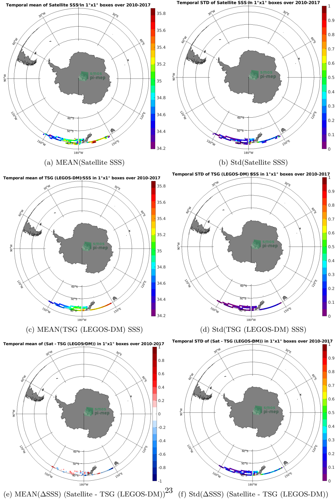
Figure 6: Temporal mean (left) and Std (right) of SSS from SMOS SSS L3 v2 - Monthly - 0.25 Deg (CATDS-CECOS-IFREMER) (top), TSG (LEGOS-DM) (middle), and of \Delta SSS (Satellite - TSG (LEGOS-DM)). Only match-up pairs are used to generate these maps.
