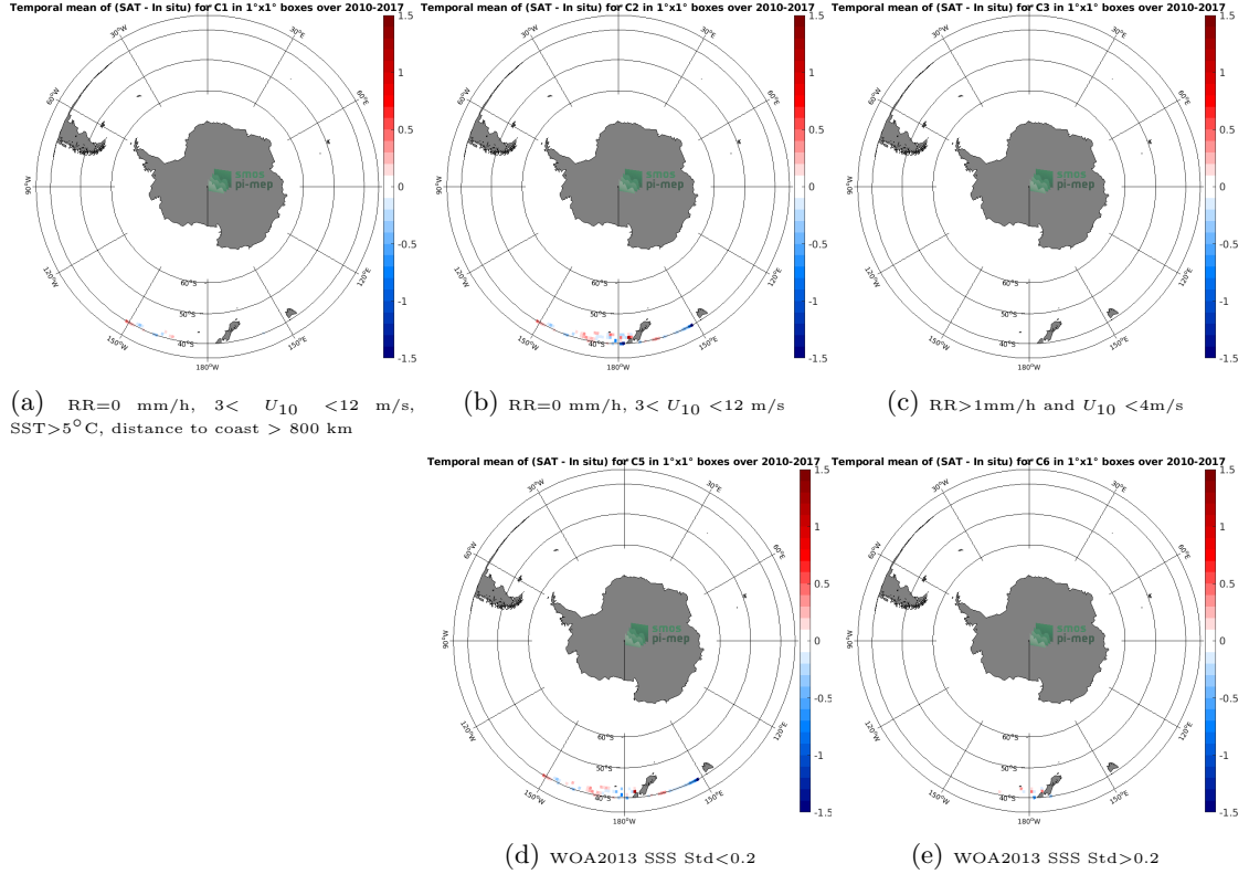
Figure 12: Temporal mean gridded over spatial boxes of size 1^{\circ}\times 1^{\circ} of \Delta\text{SSS} (SMOS SSS L3 v2 - Monthly - 0.25 Deg (CATDS-CECOS-IFREMER) - TSG (LEGOS-DM)) for 5 different subdatasets corresponding to:RR=0 mm/h, 3 < U_{10} < 12 m/s, SST >5^{\circ}\text{C} , distance to coast > 800 km (a), RR=0 mm/h, 3 < U_{10} < 12 m/s (b), RR >1 mm/h and U_{10} < 4 m/s (c), WOA2013 SSS Std <0.2 (d), WOA2013 SSS Std >0.2 (e).
