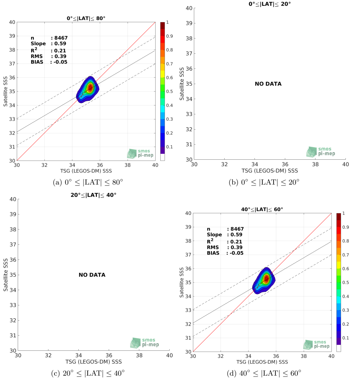
Figure 9: Contour maps of the concentration of SMOS SSS L3 v2 - Monthly - 0.25 Deg (CATDS-CECOS-IFREMER) SSS (y-axis) versus TSG (LEGOS-DM) SSS (x-axis) at match-up pairs for different latitude bands. For each plot, the red line shows x=y . The black thin and dashed lines indicate a linear fit through the data cloud and the \pm 95\% confidence levels, respectively. The number match-up pairs n , the slope and R^2 coefficient of the linear fit, the root mean square (RMS) and the mean bias between satellite and in situ data are indicated for each latitude band in each plots.
