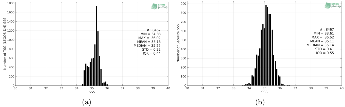
Figure 2: Histograms of SSS from TSG (LEGOS-DM) (a) and SMOS SSS L3 v2 - Monthly - 0.25 Deg (CATDS-CECOS-IFREMER) (b) considering all match-up pairs per bins of 0.1 over the Roaring Forties and Furious Fifties Pi-MEP region and for the full satellite product period.
