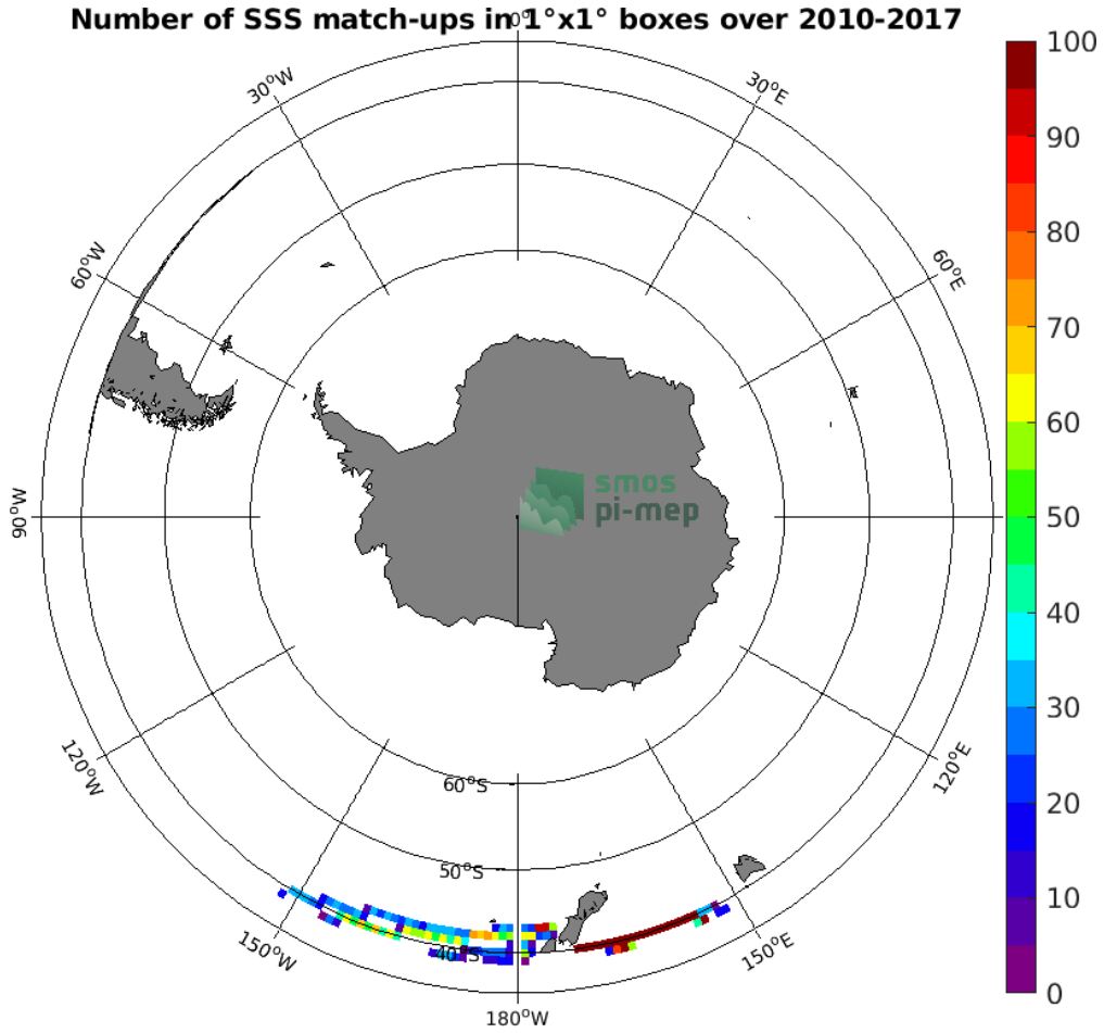
Figure 4: Number of SSS match-ups between TSG (LEGOS-DM) SSS and the SMOS SSS L3 v2 - Monthly - 0.25 Deg (CATDS-CECOS-IFREMER) SSS product for the Roaring Forties and Furious Fifties Pi-MEP region over 1^\circ \times 1^\circ boxes and for the full satellite product period.
