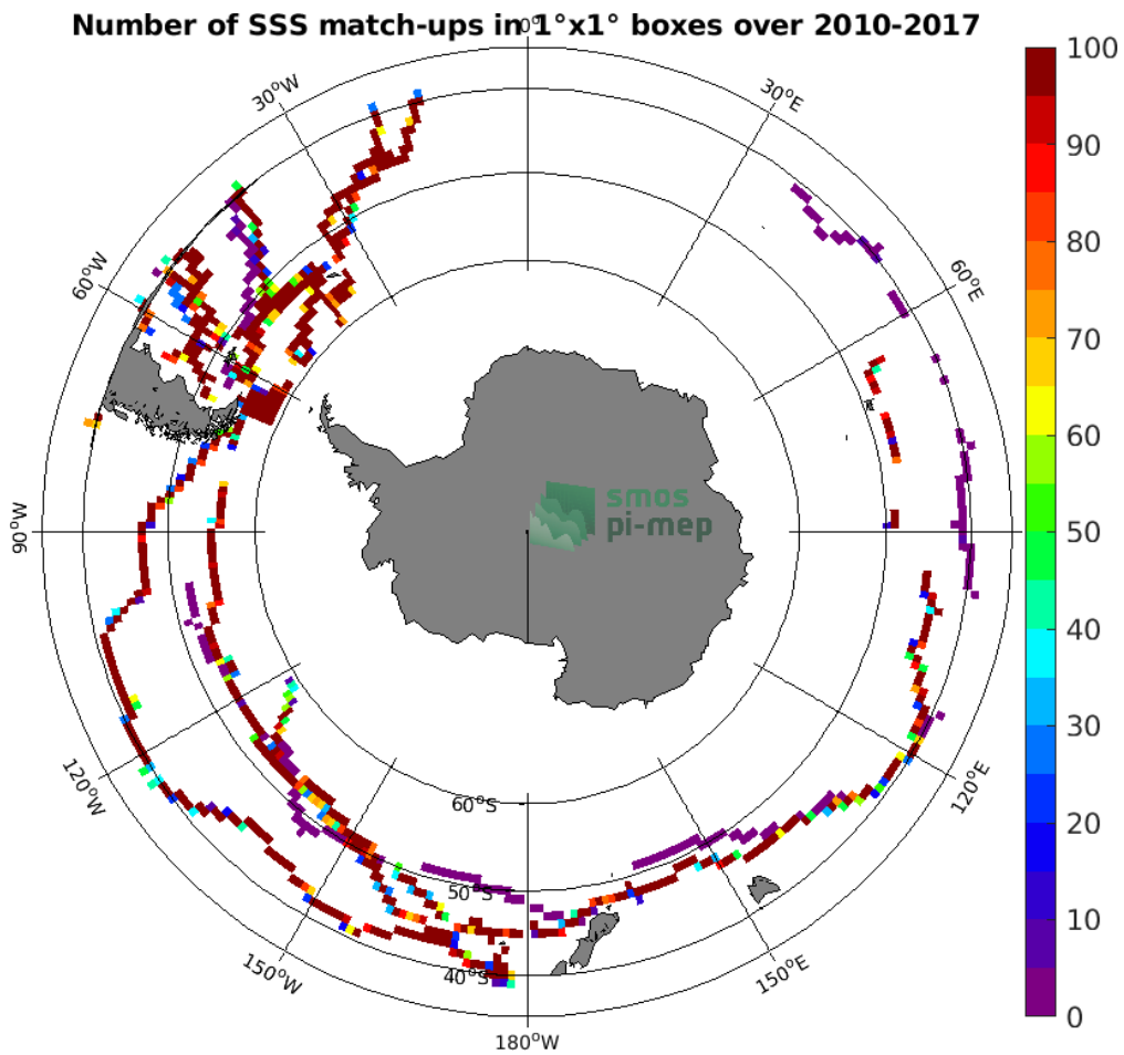
Figure 4: Number of SSS match-ups between TSG (GOSUD-Sailing-ship) SSS and the SMOS SSS L3 v2 - Monthly - 0.25 Deg (CATDS-CECOS-IFREMER) SSS product for the Roaring Forties and Furious Fifties Pi-MEP region over 1^{\circ} \times 1^{\circ} boxes and for the full satellite product period.
