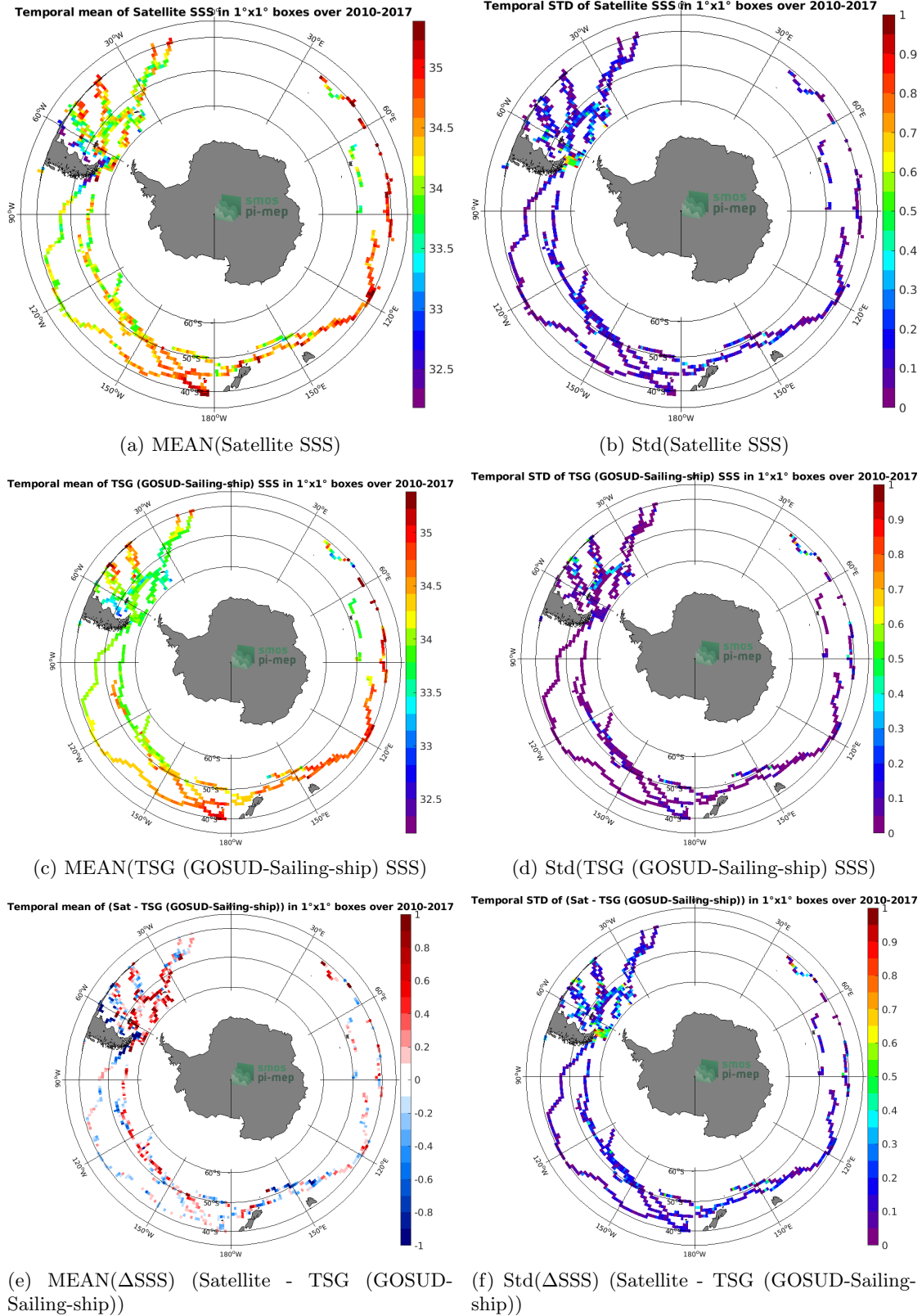
Figure 6: Temporal mean (left) and Std (right), of SSS from SMOS SSS L3 v2 - Monthly - 0.25 Deg (CATDS-CECOS-IFREMER) (top), TSG (GOSUD-Sailing-ship) (middle), and of \Delta SSS (Satellite - TSG (GOSUD-Sailing-ship)). Only match-up pairs are used to generate these maps.
