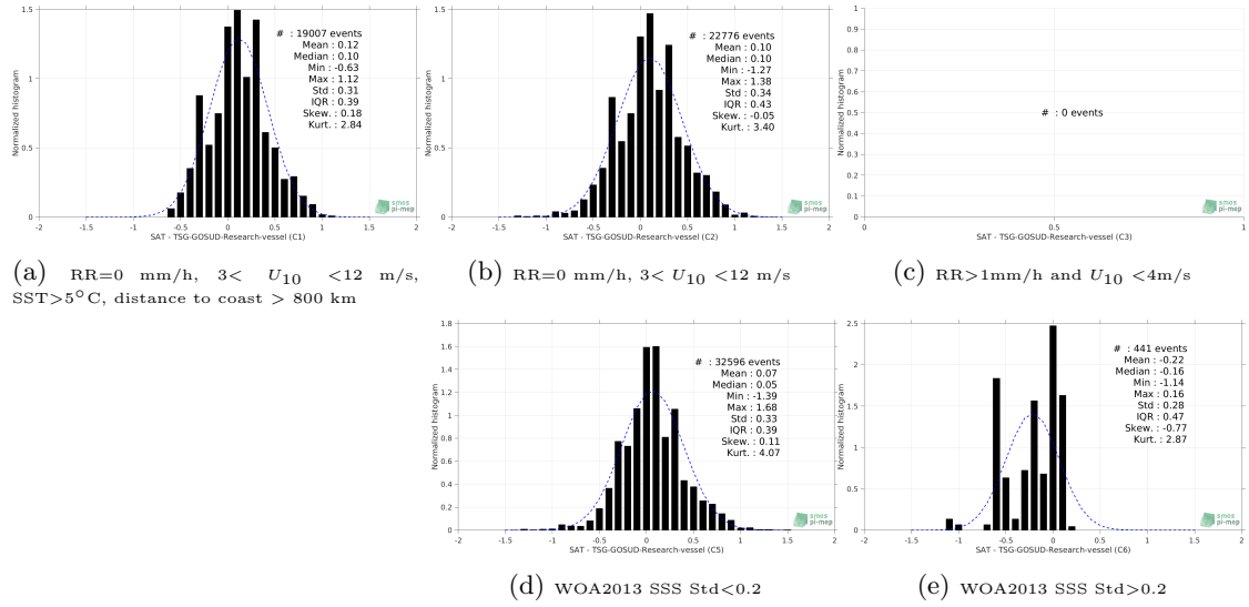
Figure 13: Normalized histogram of \Delta SSS (SMOS-L3-CATDS-IFREMER-CECOS-V2-MONTHLY-0.25DEG - TSG-GOSUD-Research-vessel) for 5 different subdatasets corresponding to: RR=0 mm/h, 3 < U_{10} < 12 m/s, SST>5°C, distance to coast > 800 km (a), RR=0 mm/h, 3 < U_{10} < 12 m/s (b), RR>1mm/h and U_{10} < 4 m/s (c), WOA2013 SSS Std<0.2 (d), WOA2013 SSS Std>0.2 (e).
