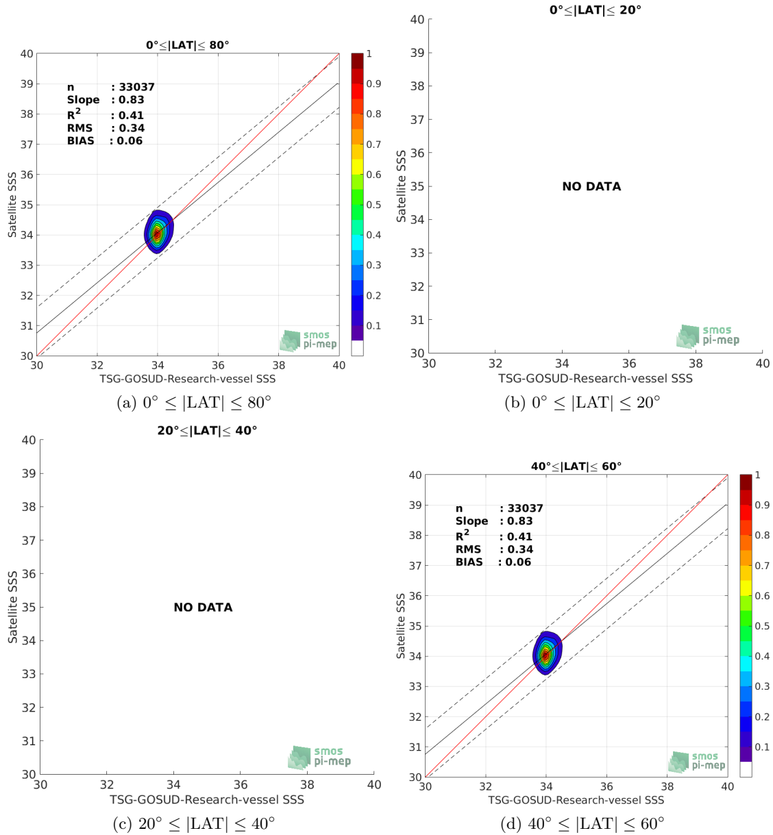
Figure 9: Contour maps of the concentration of SMOS-L3-CATDS-IFREMER-CECOS-V2-MONTHLY-0.25DEG SSS ( y -axis) versus TSG-GOSUD-Research-vessel SSS ( x -axis) at match-up pairs for different latitude bands. For each plot, the red line shows x=y . The black thin and dashed lines indicate a linear fit through the data cloud and the \pm 95\% confidence levels, respectively. The number match-up pairs n , the slope and R^2 coefficient of the linear fit, the root mean square (RMS) and the mean bias between satellite and in situ data are indicated for each latitude band in each plots.
