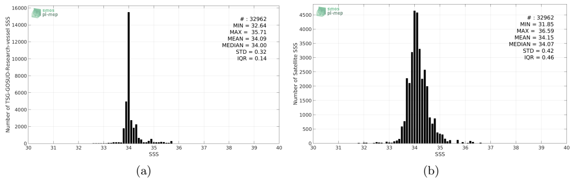
Figure 2: Histograms of SSS from TSG-GOSUD-Research-vessel (a) and SMOS-L3-CATDS-IFREMER-CECOS-V2-MONTHLY-0.25DEG (b) considering all match-up pairs per bins of 0.1 over the Roaring Forties and Furious Fifties Pi-MEP region and for the full satellite product period.
