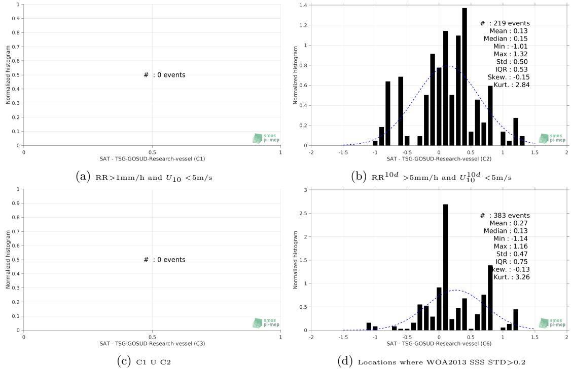
Figure 13: Normalized histogram of \Delta\text{SSS} (SMOS-L3-CATDS-IFREMER-CECOS-V2-MONTHLY-0.25DEG - TSG-GOSUD-Research-vessel) for 6 different subdatasets corresponding to: RR > 1\text{mm/h} and U_{10} < 5\text{m/s} (a), RR^{10d} > 5\text{mm/h} and U_{10}^{10d} < 5\text{m/s} (b), C1 \cup C2 (c), Locations where WOA2013 SSS STD > 0.2 (d).
