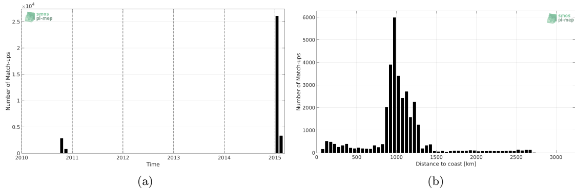
Figure 1: Number of match-ups between TSG-GOSUD-Research-vessel and SMOS-L3-CATDS-IFREMER-CECOS-V2-MONTHLY-0.25DEG SSS as a function of time (a) and as function of the distance to coast (b) over the Roaring Forties and Furious Fifties Pi-MEP region and for the full satellite product period.
