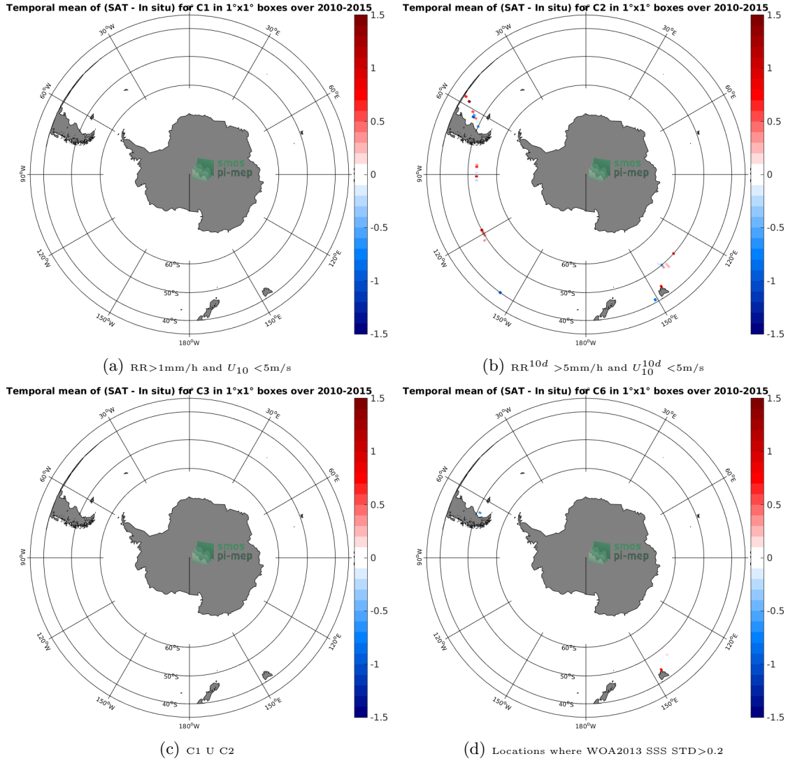
Figure 12: Temporal mean gridded over spatial boxes of size 1^\circ \times 1^\circ of \Delta SSS (SMOS-L3-CATDS-IFREMER-CECOS-V2-MONTHLY-0.25DEG - TSG-GOSUD-Research-vessel) for 4 different subdatasets corresponding to: RR > 1mm/h and U_{10} < 5\text{m/s} (a), RR^{10d} > 5\text{mm/h} and U_{10}^{10d} < 5\text{m/s} (b), C1 U C2 (c), Locations where WOA2013 SSS STD > 0.2 (d).
