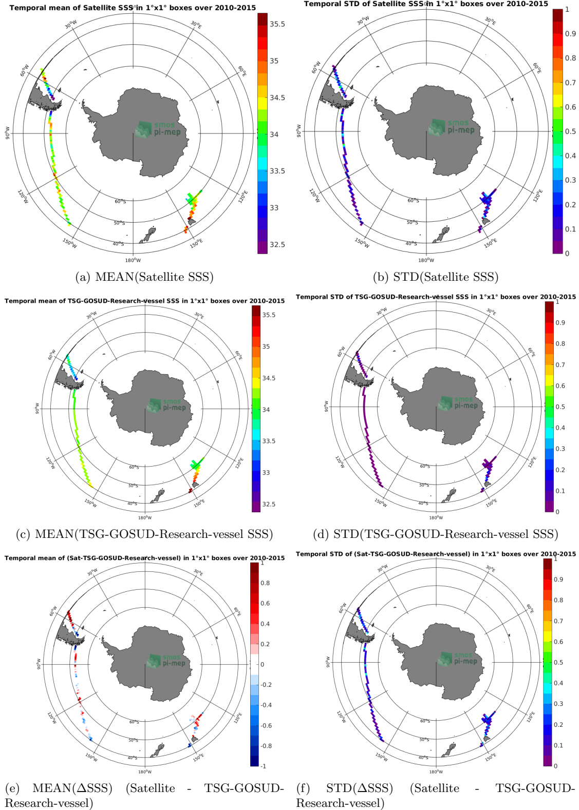
Figure 6: Temporal mean (left) and STD (right) of SSS from SMOS-L3-CATDS-IFREMER-CECOS-V2-MONTHLY-0.25DEG (top), TSG-GOSUD-Research-vessel (middle), and of \Delta SSS (Satellite - TSG-GOSUD-Research-vessel). Only match-up pairs are used to generate these maps.
