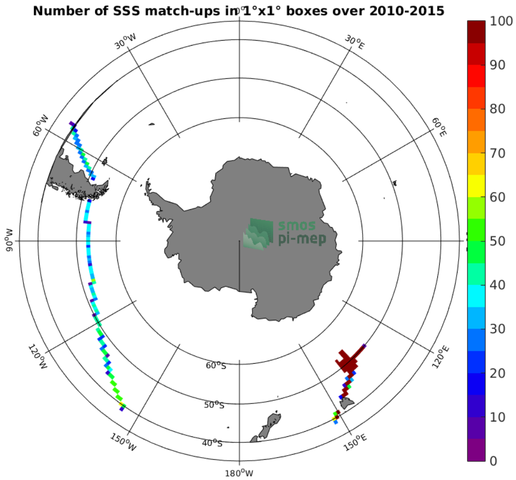
Figure 4: Number of SSS match-ups between TSG-GOSUD-Research-vessel SSS and the SMOS-L3-CATDS-IFREMER-CECOS-V2-MONTHLY-0.25DEG SSS product for the Roaring Forties and Furious Fifties Pi-MEP region over 1°x1° boxes and for the full satellite product period.
