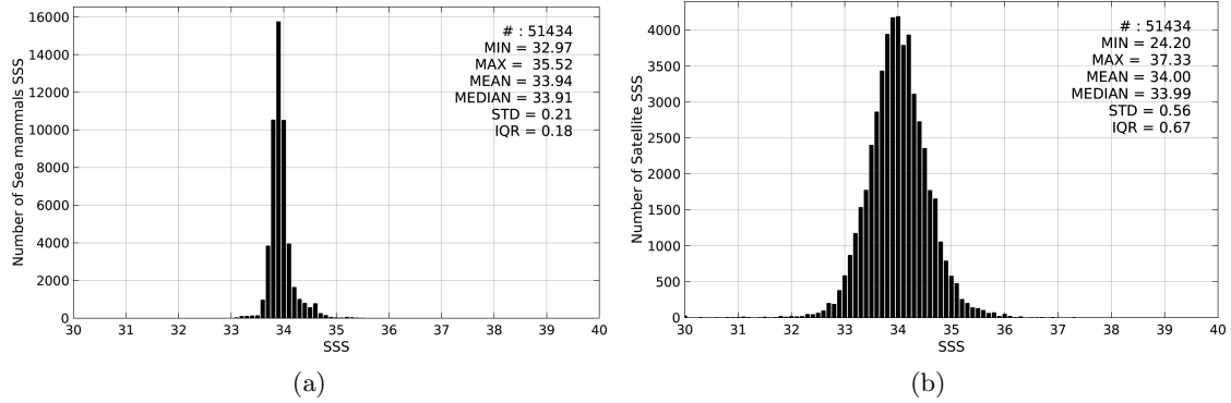
Figure 2: Histograms of SSS from Sea mammals (a) and SMOS-L3-CATDS-IFREMER-CECOS-V2-MONTHLY-0.25DEG (b) considering all match-up pairs per bins of 0.1 over the Roaring Forties and Furious Fifties Pi-MEP region and for the full satellite product period.
