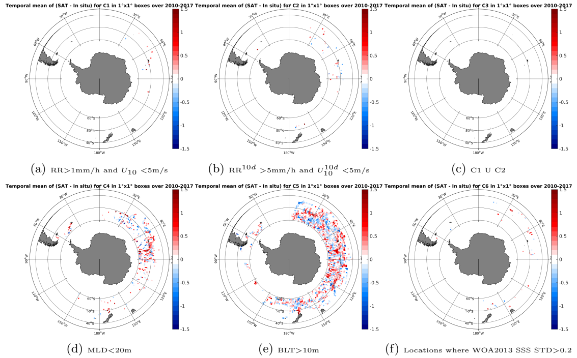
Figure 12: Temporal mean gridded over spatial boxes of size 1^\circ \times 1^\circ of \Delta SSS (SMOS-L3-CATDS-IFREMER-CECOS-V2-MONTHLY-0.25DEG - Sea mammals) for 6 different subdatasets corresponding to: RR > 1 \text{ mm/h} and U_{10} < 5 \text{ m/s} (a), RR^{10d} > 5 \text{ mm/h} and U_{10}^{10d} < 5 \text{ m/s} (b), C1 U C2 (c), MLD < 20 \text{ m} (d), BLT > 10 \text{ m} (e), Locations where WOA2013 SSS STD > 0.2 (f).
