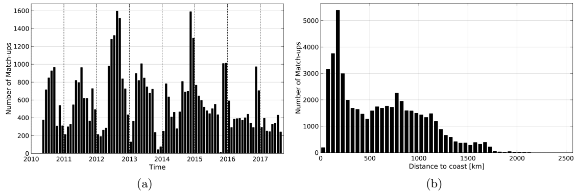
Figure 1: Number of match-ups between Sea mammals and SMOS-L3-CATDS-IFREMER-CECOS-V2-MONTHLY-0.25DEG SSS as a function of time (a) and as function of the distance to coast (b) over the Roaring Forties and Furious Fifties Pi-MEP region and for the full satellite product period.
