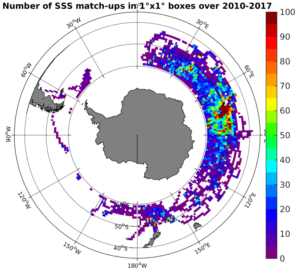
Figure 4: Number of SSS match-ups between Sea mammals SSS and the SMOS-L3-CATDS-IFREMER-CECOS-V2-MONTHLY-0.25DEG SSS product for the Roaring Forties and Furious Fifties Pi-MEP region over 1^\circ \times 1^\circ boxes and for the full satellite product period.
