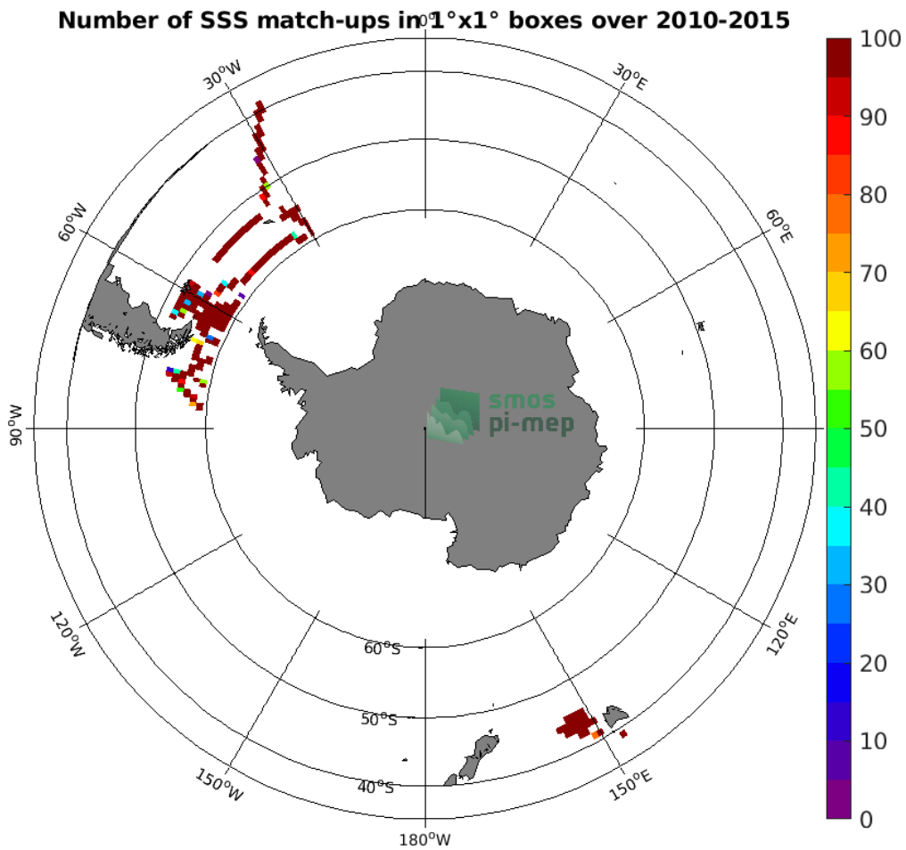
Figure 4: Number of SSS match-ups between TSG (SAMOS) SSS and the SMOS SSS L3 v2 - Daily - 0.5 Deg (CATDS-CECOS-IFREMER) SSS product for the Roaring Forties and Furious Fifties Pi-MEP region over 1^\circ \times 1^\circ boxes and for the full satellite product period.
