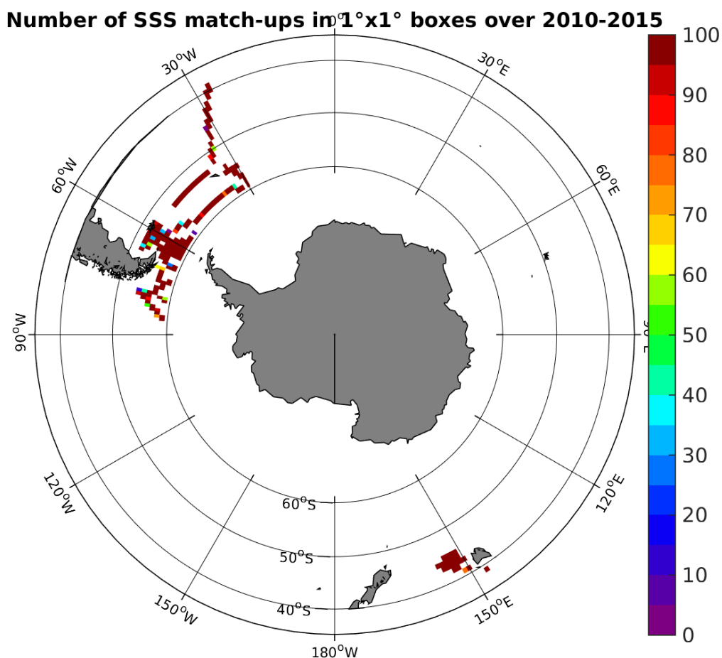
Figure 4: Number of SSS match-ups between TSG-SAMOS SSS and the SMOS-L3-CATDS-CECOS-IFREMER-V2-1DAY-0.5DEG SSS product for the Roaring Forties and Furious Fifties Pi-MEP region over 1°x1° boxes and for the full satellite product period.
