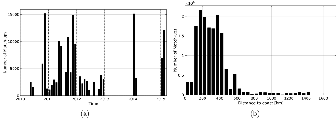
Figure 1: Number of match-ups between TSG-SAMOS and SMOS-L3-CATDS-CECOS-IFREMER-V2-1DAY-0.5DEG SSS as a function of time (a) and as function of the distance to coast (b) over the Roaring Forties and Furious Fifties Pi-MEP region and for the full satellite product period.
