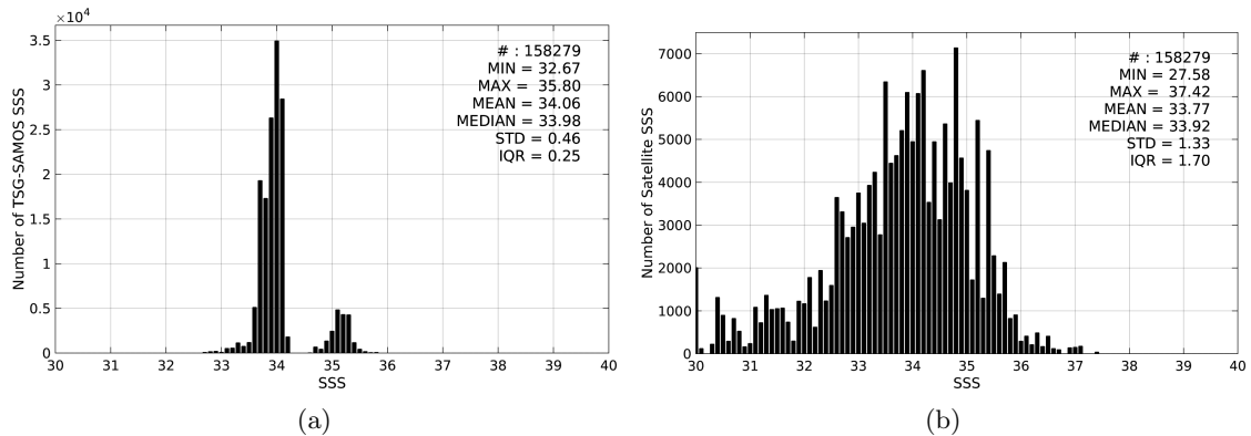
Figure 2: Histograms of SSS from TSG-SAMOS (a) and SMOS-L3-CATDS-CECOS-IFREMER-V2-1DAY-0.5DEG (b) considering all match-up pairs per bins of 0.1 over the Roaring Forties and Furious Fifties Pi-MEP region and for the full satellite product period.
