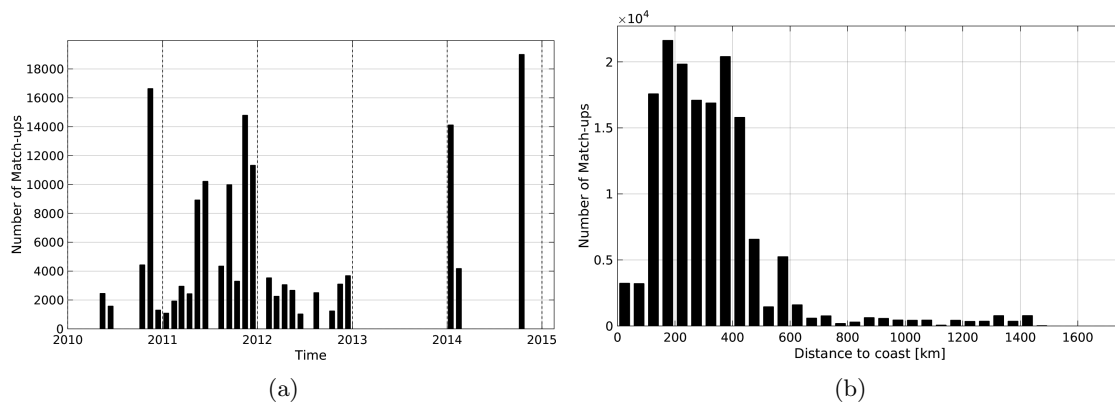
Figure 1: Number of match-ups between TSG-SAMOS and SMOS-L3-CATDS-CECOS-IFREMER-V2-1DAY-0.5deg SSS as a function of time (a) and as function of the distance to coast (b) over the Roaring Forties and Furious Fifties Pi-MEP region and for the full satellite product period.
