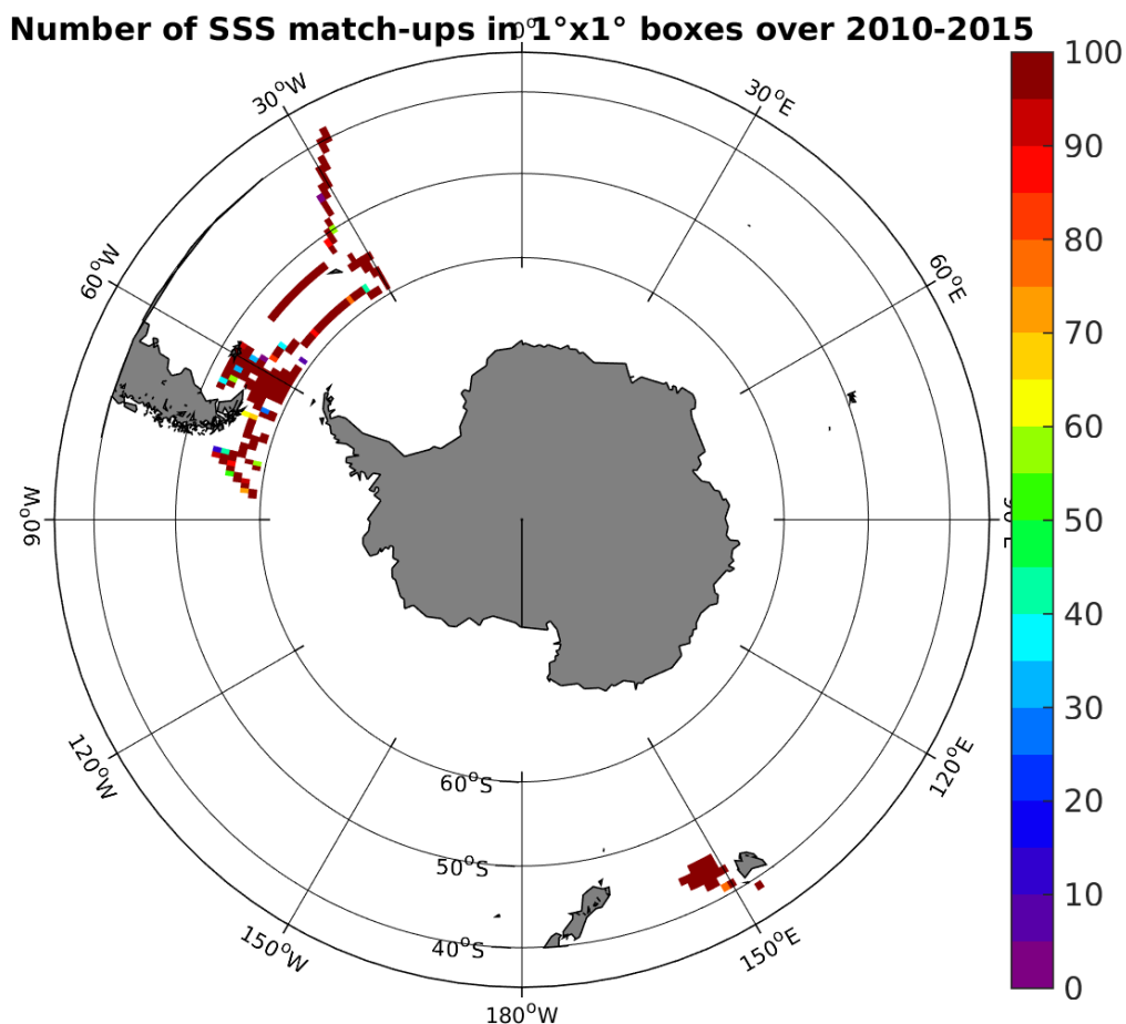
Figure 4: Number of SSS match-ups between TSG-SAMOS SSS and the SMOS-L3-CATDS-CECOS-IFREMER-V2-1DAY-0.5deg SSS product for the Roaring Forties and Furious Fifties Pi-MEP region over 1^\circ \times 1^\circ boxes and for the full satellite product period.
