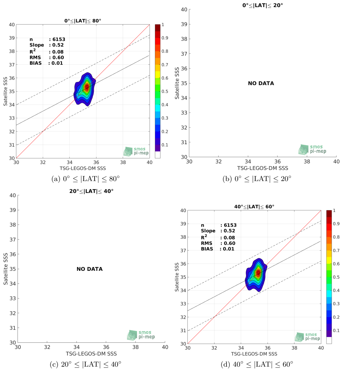
Figure 9: Contour maps of the concentration of SMOS L3 v2 - Daily - 0.5 Deg (CATDS-CECOS-IFREMER) SSS (y-axis) versus TSG-LEGOS-DM SSS (x-axis) at match-up pairs for different latitude bands. For each plot, the red line shows x=y . The black thin and dashed lines indicate a linear fit through the data cloud and the \pm 95\% confidence levels, respectively. The number match-up pairs n , the slope and R^2 coefficient of the linear fit, the root mean square (RMS) and the mean bias between satellite and in situ data are indicated for each latitude band in each plots.
