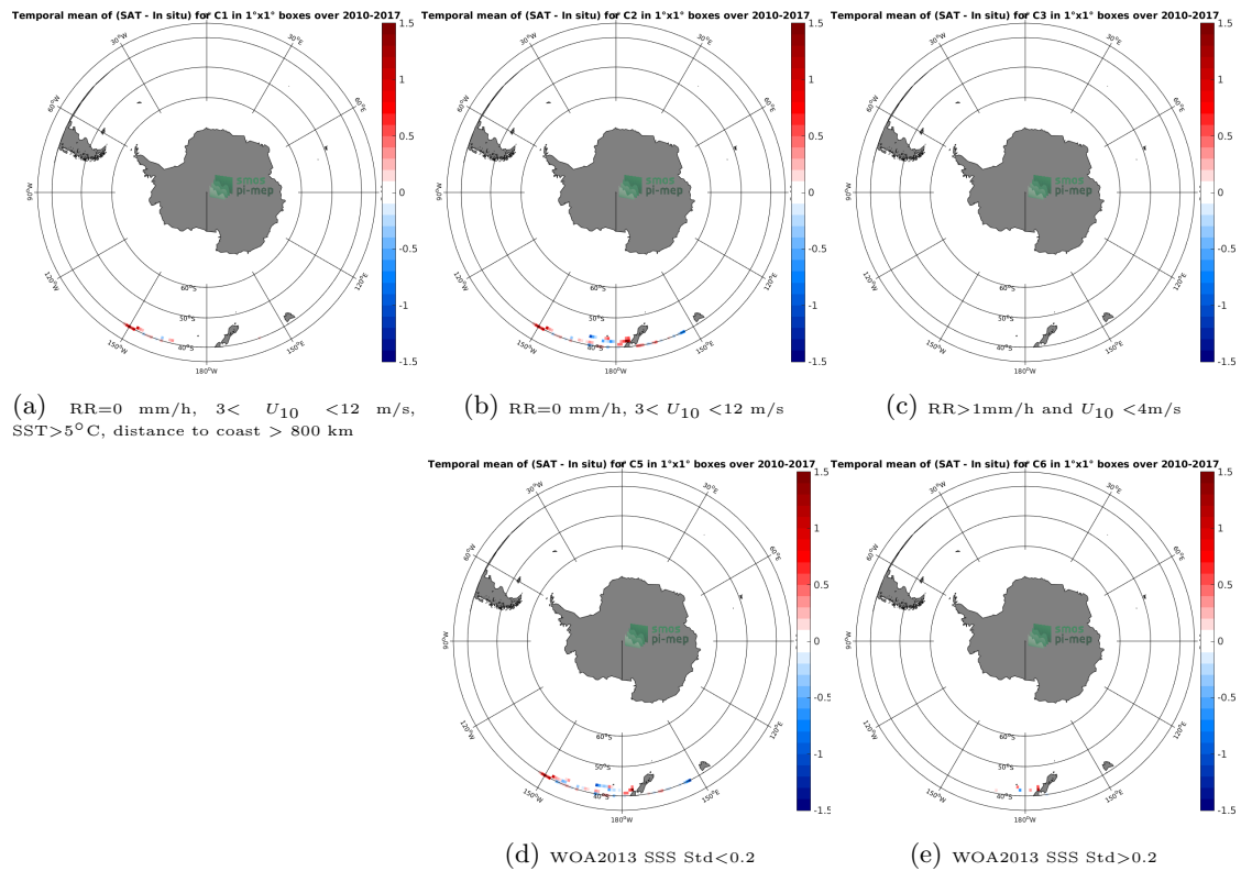
Figure 12: Temporal mean gridded over spatial boxes of size 1^{\circ}\times 1^{\circ} of \Delta\text{SSS} (SMOS L3 v2 - Daily - 0.5 Deg (CATDS-CECOS-IFREMER) - TSG-LEGOS-DM) for 5 different subdatasets corresponding to:RR=0 mm/h, 3 < U_{10} < 12 m/s, SST >5^{\circ}\text{C} , distance to coast > 800 km (a), RR=0 mm/h, 3 < U_{10} < 12 m/s (b), RR >1 mm/h and U_{10} < 4 m/s (c), WOA2013 SSS Std <0.2 (d), WOA2013 SSS Std >0.2 (e).
