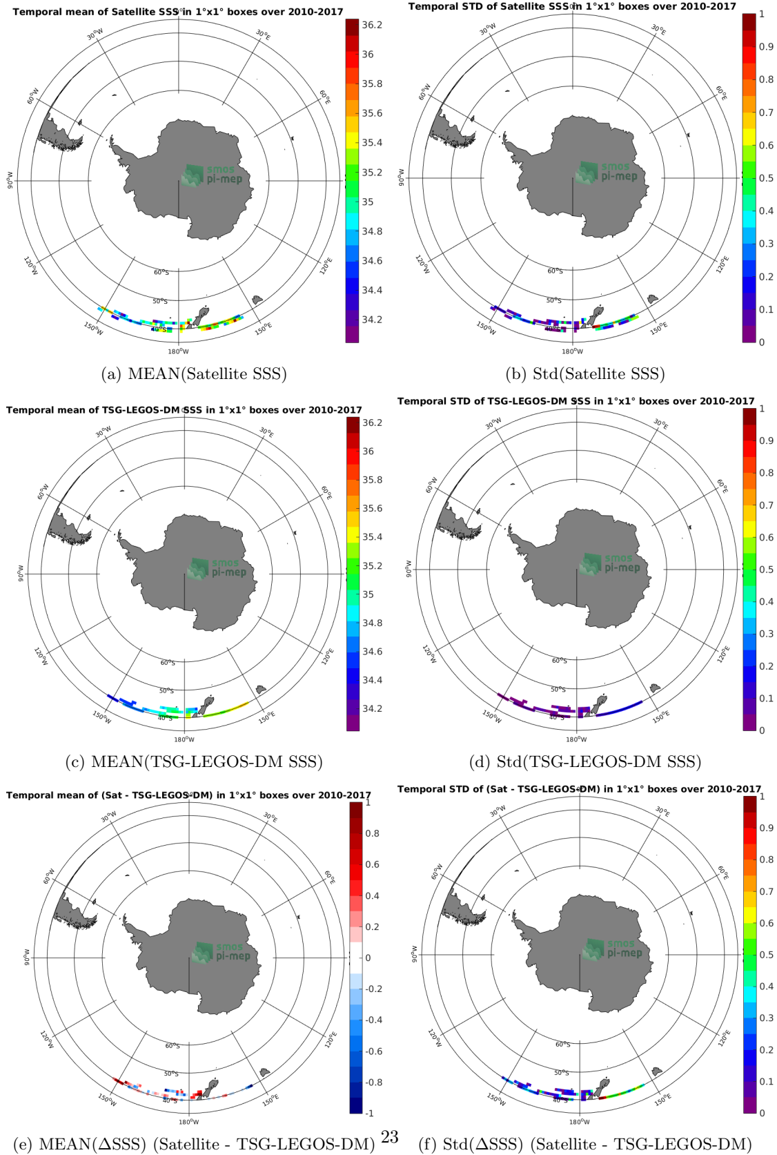
Figure 6: Temporal mean (left) and Std (right) of SSS from SMOS L3 v2 - Daily - 0.5 Deg (CATDS-CECOS-IFREMER) (top), TSG-LEGOS-DM (middle), and of \Delta SSS (Satellite - TSG-LEGOS-DM). Only match-up pairs are used to generate these maps.
