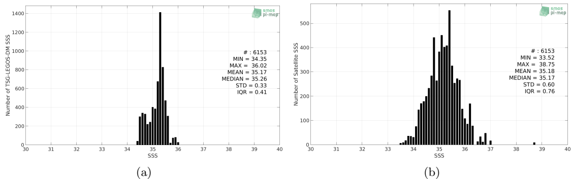
Figure 2: Histograms of SSS from TSG-LEGOS-DM (a) and SMOS L3 v2 - Daily - 0.5 Deg (CATDS-CECOS-IFREMER) (b) considering all match-up pairs per bins of 0.1 over the Roaring Forties and Furious Fifties Pi-MEP region and for the full satellite product period.
