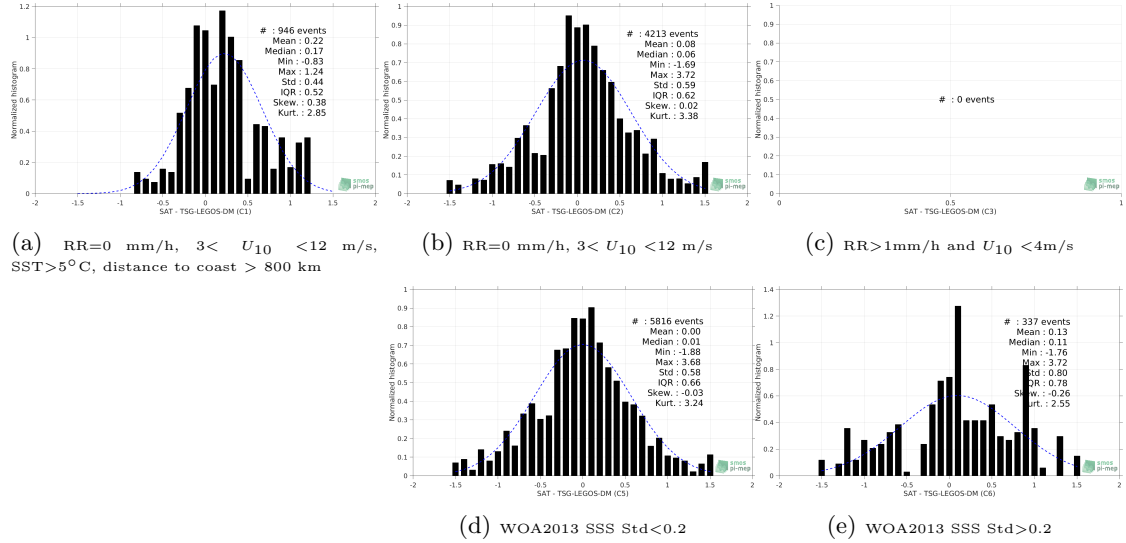
Figure 13: Normalized histogram of \Delta SSS (SMOS L3 v2 - Daily - 0.5 Deg (CATDS-CECOS-IFREMER) - TSG-LEGOS-DM) for 5 different subdatasets corresponding to: RR=0 mm/h, 3 < U_{10} < 12 m/s, SST > 5°C, distance to coast > 800 km (a), RR=0 mm/h, 3 < U_{10} < 12 m/s (b), RR > 1mm/h and U_{10} < 4 m/s (c), WOA2013 SSS Std < 0.2 (d), WOA2013 SSS Std > 0.2 (e).
