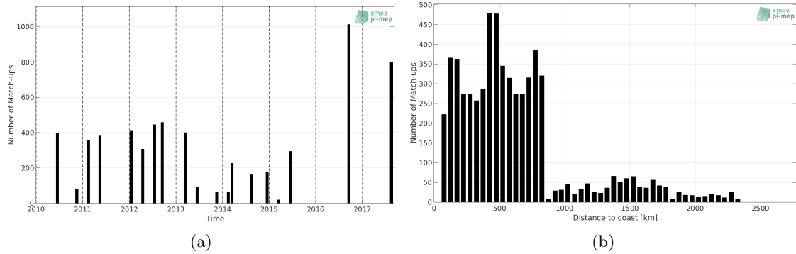
Figure 1: Number of match-ups between TSG-LEGOS-DM and SMOS L3 v2 - Daily - 0.5 Deg (CATDS-CECOS-IFREMER) SSS as a function of time (a) and as function of the distance to coast (b) over the Roaring Forties and Furious Fifties Pi-MEP region and for the full satellite product period.
