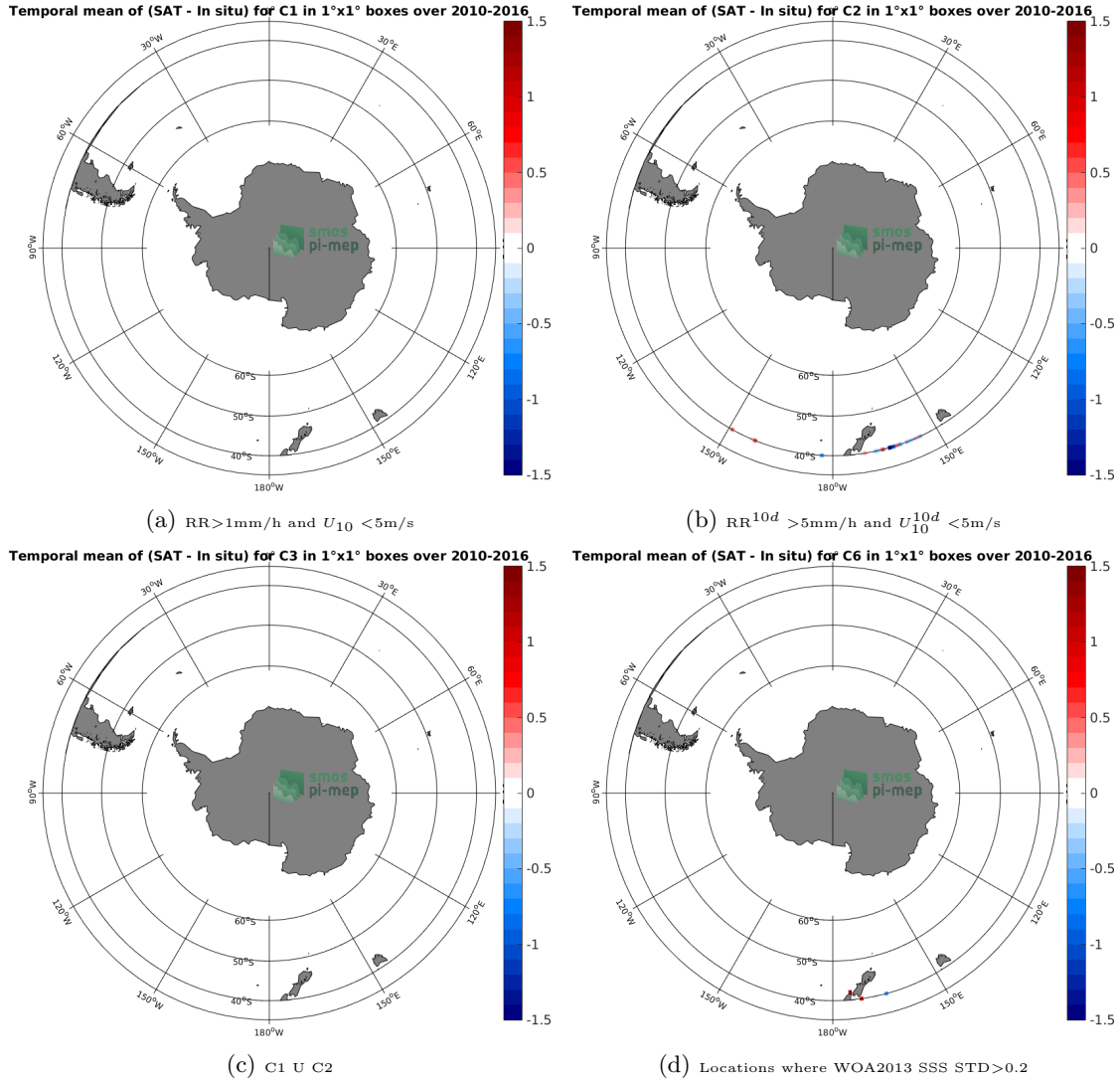
Figure 12: Temporal mean gridded over spatial boxes of size 1^\circ \times 1^\circ of \Delta SSS (SMOS-L3-CATDS-CECOS-IFREMER-V2-1DAY-0.5DEG - TSG-LEGOS-DM) for 4 different subdatasets corresponding to: RR > 1mm/h and U_{10} < 5\text{m/s} (a), RR^{10d} > 5\text{mm/h} and U_{10}^{10d} < 5\text{m/s} (b), C1 U C2 (c), Locations where WOA2013 SSS STD > 0.2 (d).
