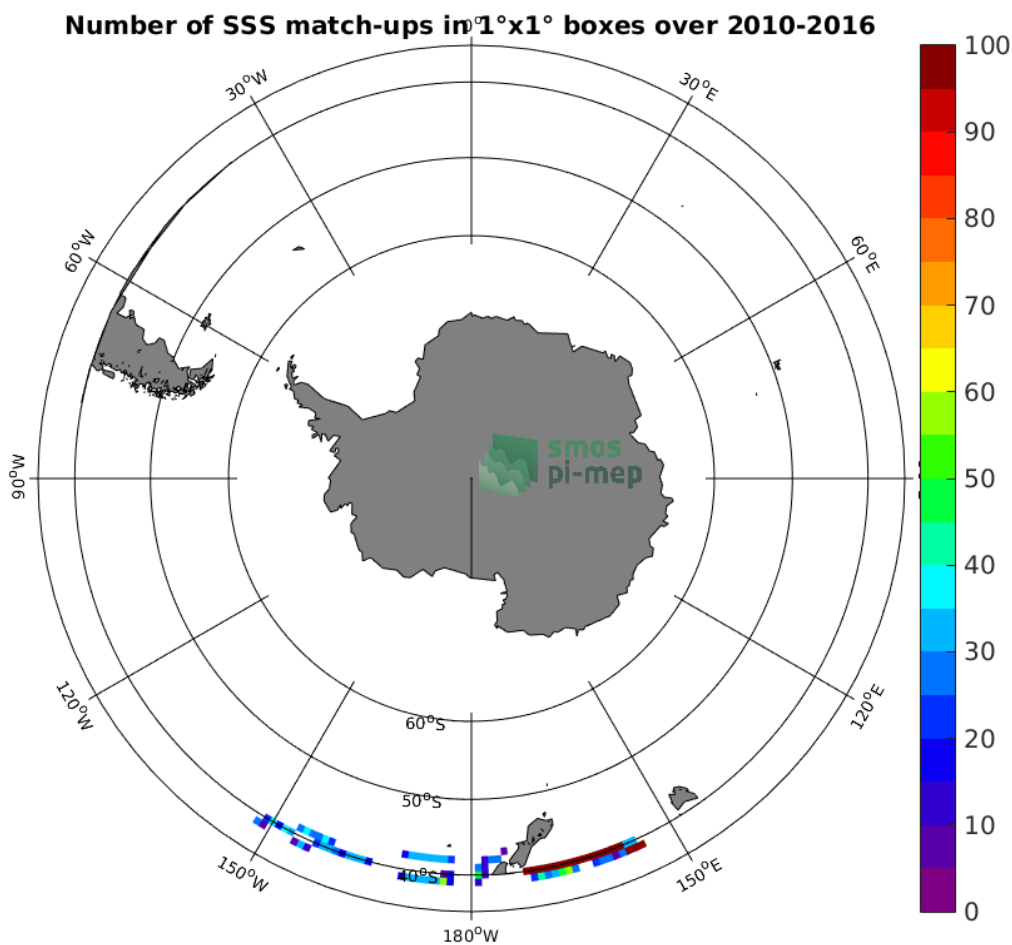
Figure 4: Number of SSS match-ups between TSG-LEGOS-DM SSS and the SMOS-L3-CATDS-CECOS-IFREMER-V2-1DAY-0.5DEG SSS product for the Roaring Forties and Furious Fifties Pi-MEP region over 1^{\circ} \times 1^{\circ} boxes and for the full satellite product period.
