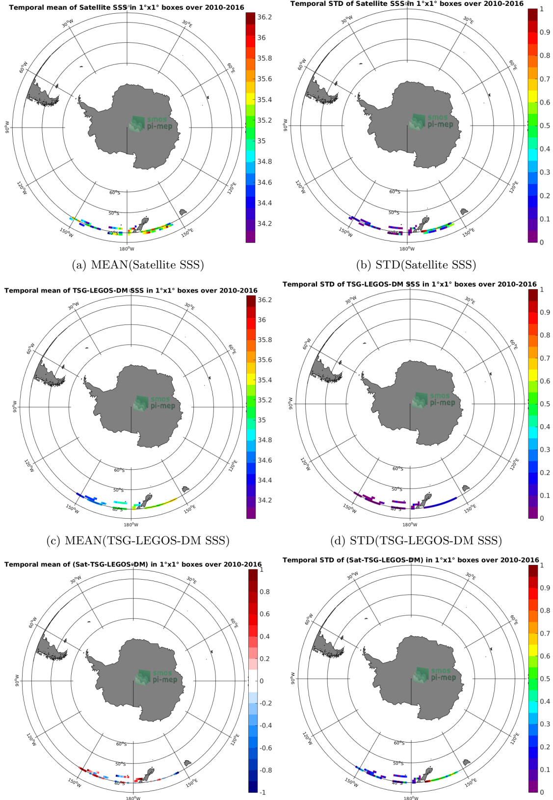
Figure 6: Temporal mean (left) and STD (right) of SSS from SMOS-L3-CATDS-CECOS-IFREMER-V2-1DAY-0.5DEG (top), TSG-LEGOS-DM (middle), and of \Delta SSS (Satellite - TSG-LEGOS-DM). Only match-up pairs are used to generate these maps.
