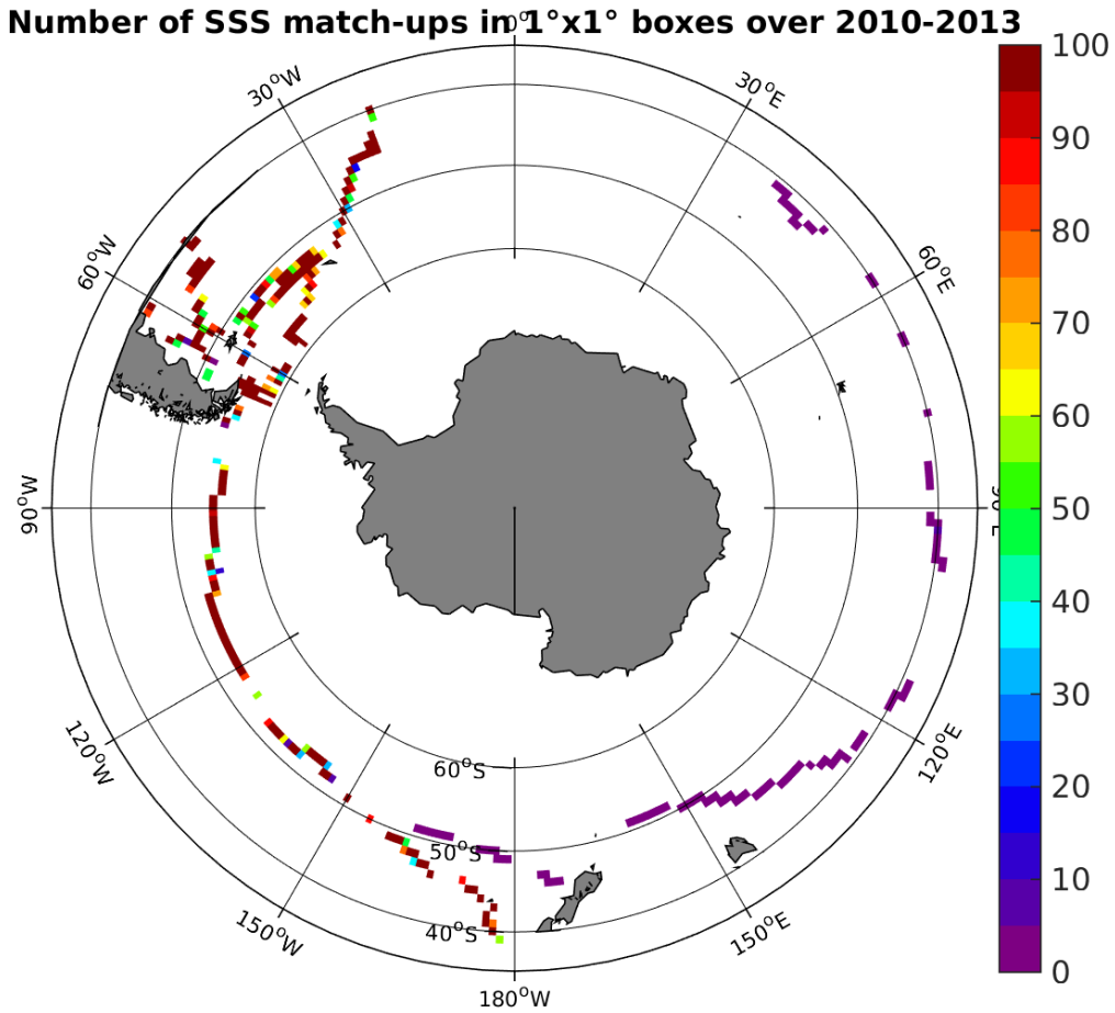
Figure 4: Number of SSS match-ups between TSG-GOSUD-Sailing-ship SSS and the SMOS-L3-CATDS-CECOS-IFREMER-V2-1DAY-0.5DEG SSS product for the Roaring Forties and Furious Fifties Pi-MEP region over 1^\circ \times 1^\circ boxes and for the full satellite product period.
