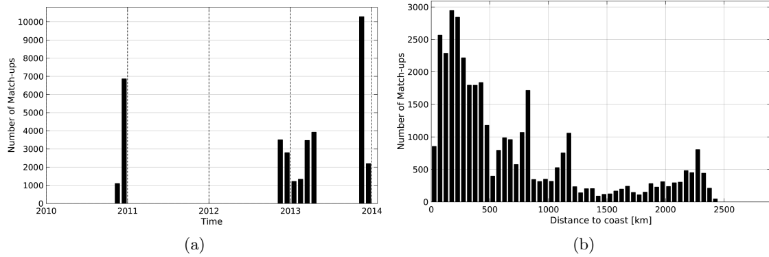
Figure 1: Number of match-ups between TSG-GOSUD-Sailing-ship and SMOS-L3-CATDS-CECOS-IFREMER-V2-1DAY-0.5DEG SSS as a function of time (a) and as function of the distance to coast (b) over the Roaring Forties and Furious Fifties Pi-MEP region and for the full satellite product period.
