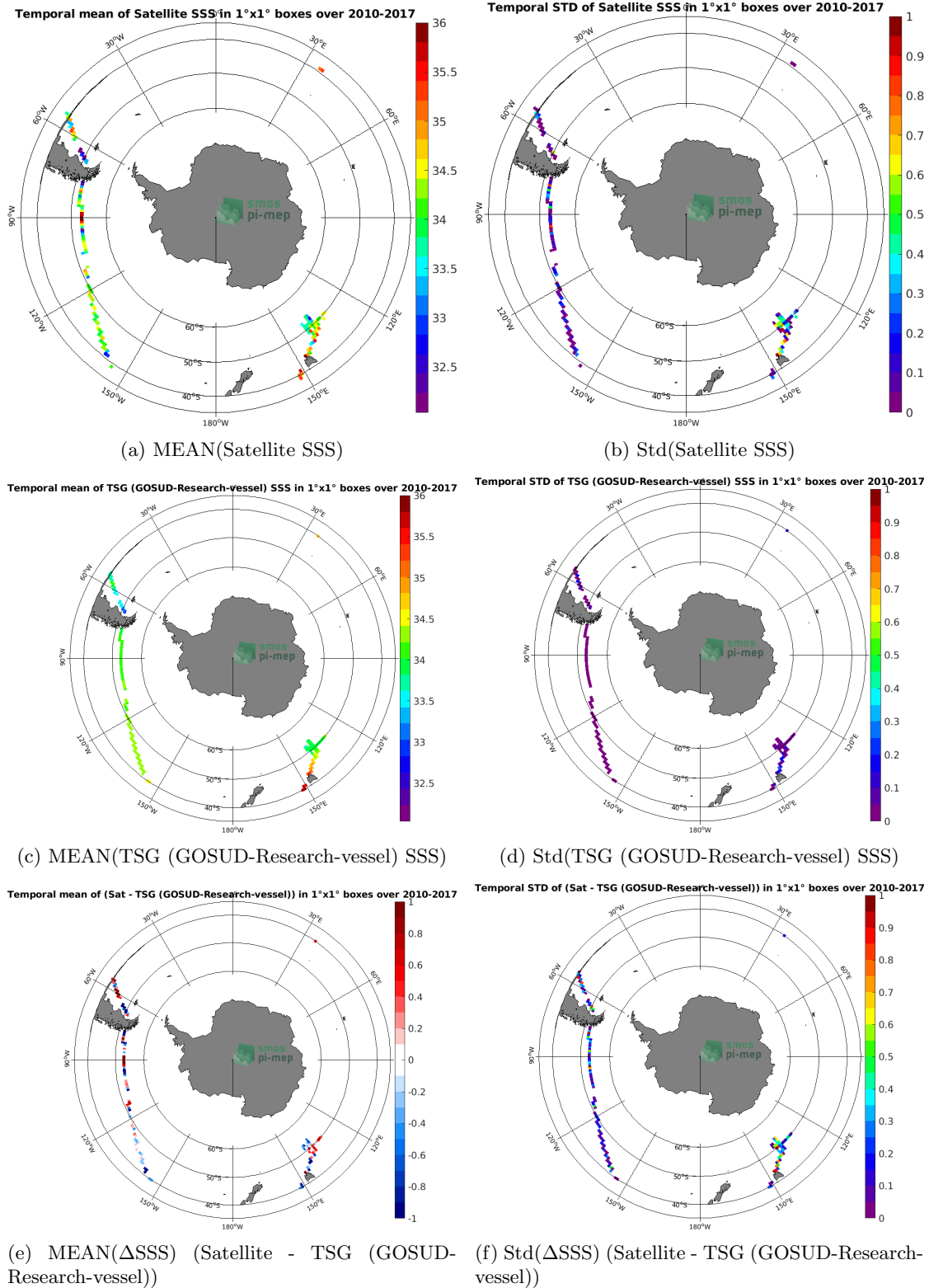
Figure 6: Temporal mean (left) and Std (right) of SSS from SMOS SSS L3 v2 - Daily - 0.5 Deg (CATDS-CECOS-IFREMER) (top), TSG (GOSUD-Research-vessel) (middle), and of \Delta SSS (Satellite - TSG (GOSUD-Research-vessel)). Only match-up pairs are used to generate these maps.
