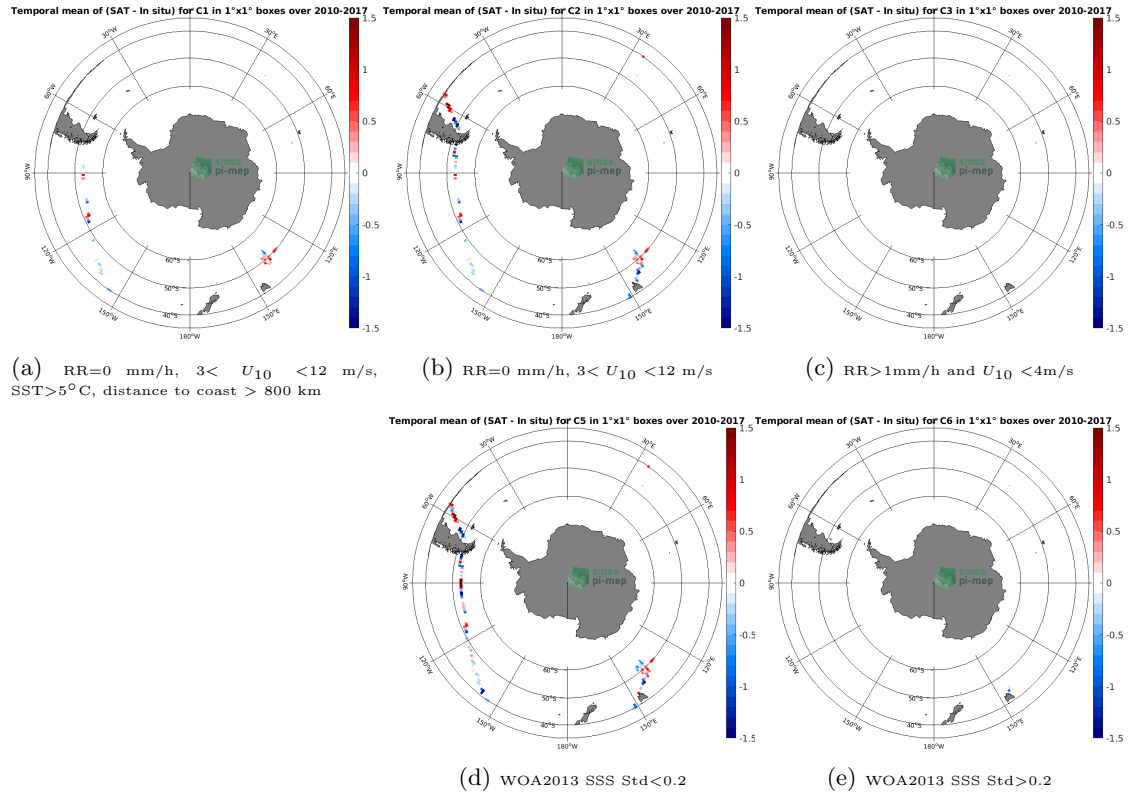
Figure 12: Temporal mean gridded over spatial boxes of size 1°x1° of \Delta SSS (SMOS SSS L3 v2 - Daily - 0.5 Deg (CATDS-CECOS-IFREMER) - TSG (GOSUD-Research-vessel)) for 5 different subdatasets corresponding to: RR=0 mm/h, 3 < U_{10} < 12 m/s, SST > 5°C, distance to coast > 800 km (a), RR=0 mm/h, 3 < U_{10} < 12 m/s (b), RR > 1mm/h and U_{10} < 4 m/s (c), WOA2013 SSS Std < 0.2 (d), WOA2013 SSS Std > 0.2 (e).
