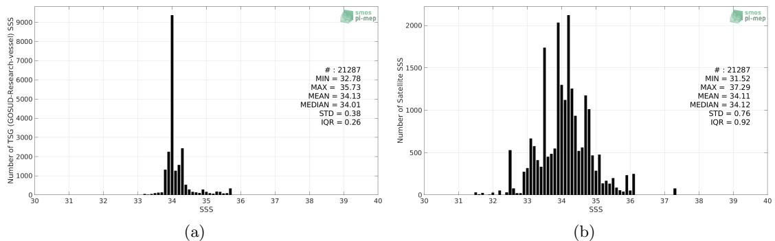
Figure 2: Histograms of SSS from TSG (GOSUD-Research-vessel) (a) and SMOS SSS L3 v2 - Daily - 0.5 Deg (CATDS-CECOS-IFREMER) (b) considering all match-up pairs per bins of 0.1 over the Roaring Forties and Furious Fifties Pi-MEP region and for the full satellite product period.
