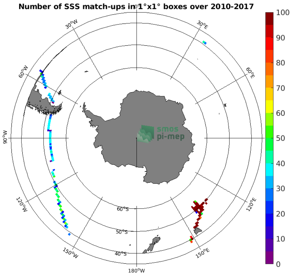
Figure 4: Number of SSS match-ups between TSG (GOSUD-Research-vessel) SSS and the SMOS SSS L3 v2 - Daily - 0.5 Deg (CATDS-CECOS-IFREMER) SSS product for the Roaring Forties and Furious Fifties Pi-MEP region over 1^\circ \times 1^\circ boxes and for the full satellite product period.
