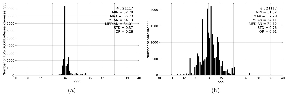
Figure 2: Histograms of SSS from TSG-GOSUD-Research-vessel (a) and SMOS-L3-CATDS-CECOS-IFREMER-V2-1DAY-0.5DEG (b) considering all match-up pairs per bins of 0.1 over the Roaring Forties and Furious Fifties Pi-MEP region and for the full satellite product period.
