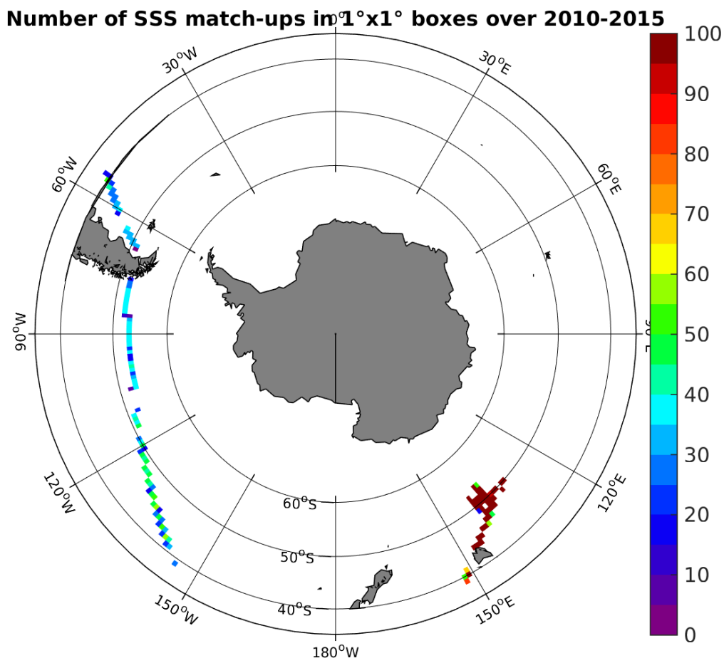
Figure 4: Number of SSS match-ups between TSG-GOSUD-Research-vessel SSS and the SMOS-L3-CATDS-CECOS-IFREMER-V2-1DAY-0.5DEG SSS product for the Roaring Forties and Furious Fifties Pi-MEP region over 1°x1° boxes and for the full satellite product period.
