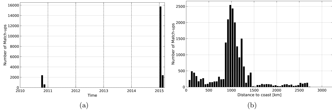
Figure 1: Number of match-ups between TSG-GOSUD-Research-vessel and SMOS-L3-CATDS-CECOS-IFREMER-V2-1DAY-0.5DEG SSS as a function of time (a) and as function of the distance to coast (b) over the Roaring Forties and Furious Fifties Pi-MEP region and for the full satellite product period.
