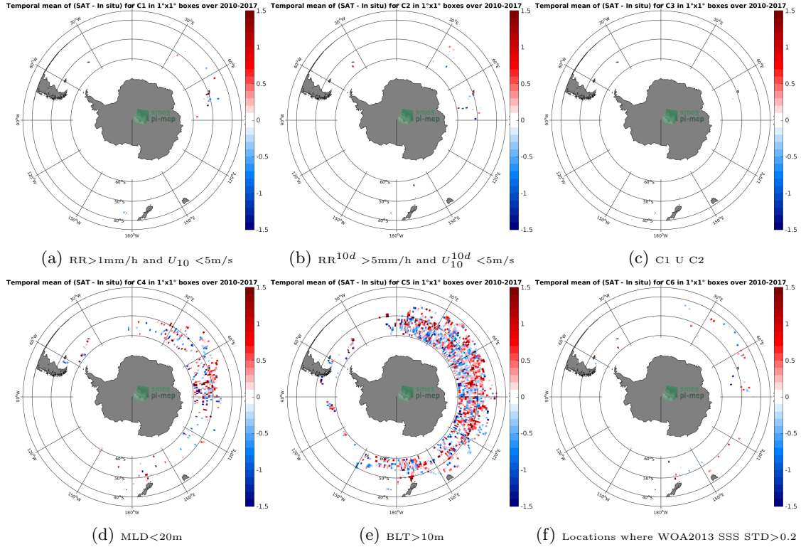
Figure 12: Temporal mean gridded over spatial boxes of size 1^\circ \times 1^\circ of \Delta SSS (SMOS-L3-CATDS-CECOS-IFREMER-V2-1DAY-0.5DEG - Sea mammals) for 6 different subdatasets corresponding to: RR > 1\text{mm/h} and U_{10} < 5\text{m/s} (a), RR^{10d} > 5\text{mm/h} and U_{10}^{10d} < 5\text{m/s} (b), C1 U C2 (c), MLD < 20\text{m} (d), BLT > 10\text{m} (e), Locations where WOA2013 SSS STD > 0.2 (f).
