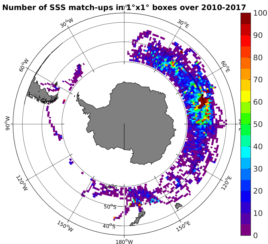
Figure 4: Number of SSS match-ups between Sea mammals SSS and the SMOS-L3-CATDS-CECOS-IFREMER-V2-1DAY-0.5DEG SSS product for the Roaring Forties and Furious Fifties Pi-MEP region over 1^\circ \times 1^\circ boxes and for the full satellite product period.
