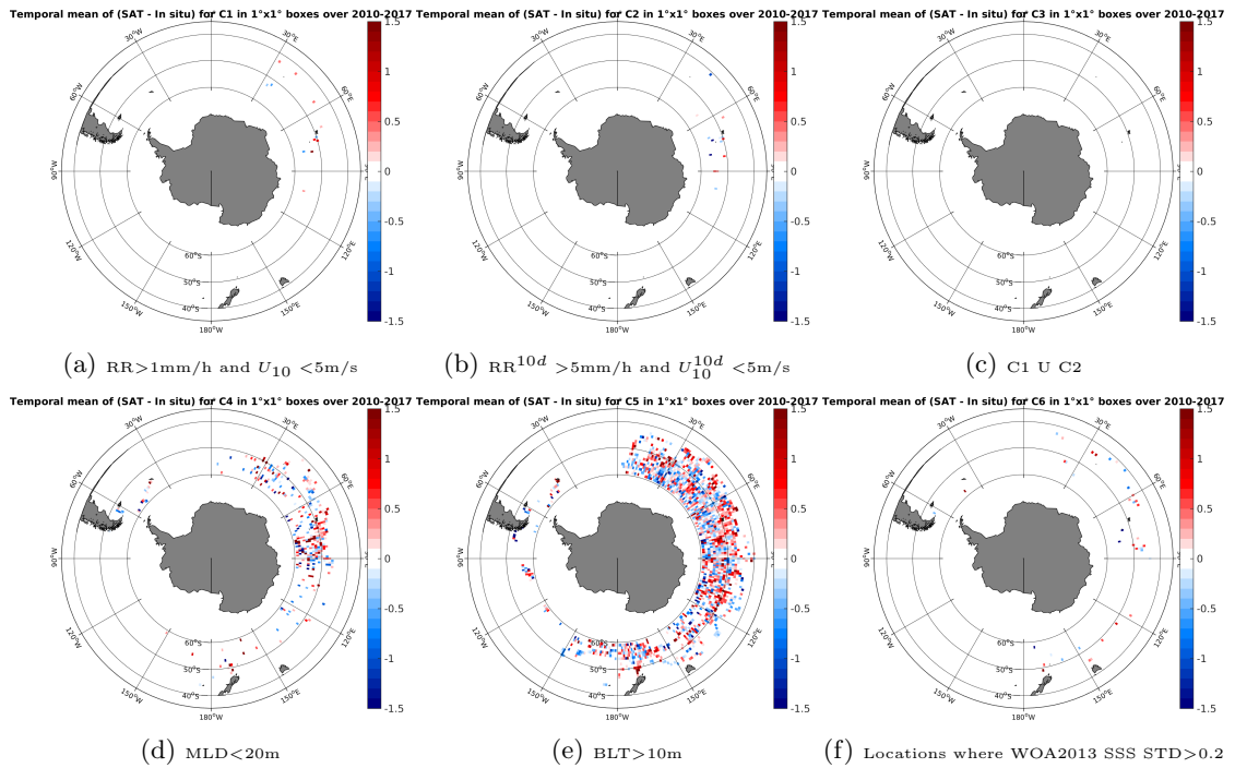
Figure 12: Temporal mean gridded over spatial boxes of size 1^\circ \times 1^\circ of \Delta SSS (SMOS-L3-CATDS-CECOS-IFREMER-V2-1DAY-0.5DEG - Sea mammals) for 6 different subdatasets corresponding to: RR > 1\text{mm/h} and U_{10} < 5\text{m/s} (a), RR^{10d} > 5\text{mm/h} and U_{10}^{10d} < 5\text{m/s} (b), C1 U C2 (c), MLD < 20\text{m} (d), BLT > 10\text{m} (e), Locations where WOA2013 SSS STD > 0.2 (f).
