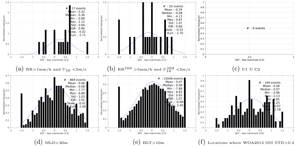
Figure 13: Normalized histogram of \Delta SSS (SMOS-L3-CATDS-CECOS-IFREMER-V2-1DAY-0.5DEG - Sea mammals) for 6 different subdatasets corresponding to: RR>1mm/h and U_{10} < 5m/s (a), RR^{10d} > 5mm/h and U_{10}^{10d} < 5m/s (b), C1 U C2 (c),MLD<20m (d),BLT>10m (e),Locations where WOA2013 SSS STD>0.2 (f).
