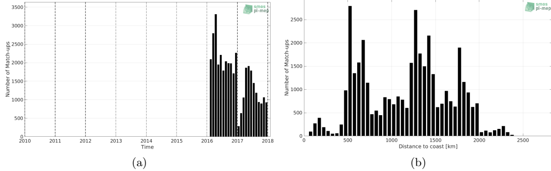
Figure 1: Number of match-ups between Surface drifters and SMOS SSS L3 v2 - Daily - 0.5 Deg (CATDS-CECOS-IFREMER) SSS as a function of time (a) and as function of the distance to coast (b) over the Roaring Forties and Furious Fifties Pi-MEP region and for the full satellite product period.
