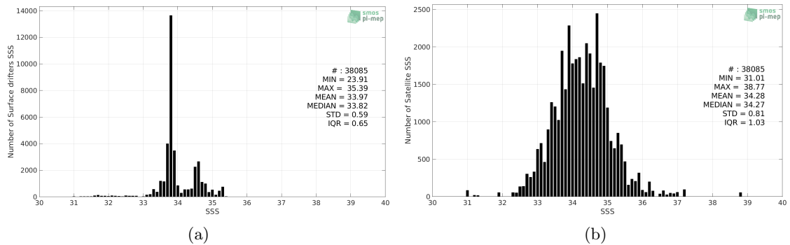
Figure 2: Histograms of SSS from Surface drifters (a) and SMOS SSS L3 v2 - Daily - 0.5 Deg (CATDS-CECOS-IFREMER) (b) considering all match-up pairs per bins of 0.1 over the Roaring Forties and Furious Fifties Pi-MEP region and for the full satellite product period.
