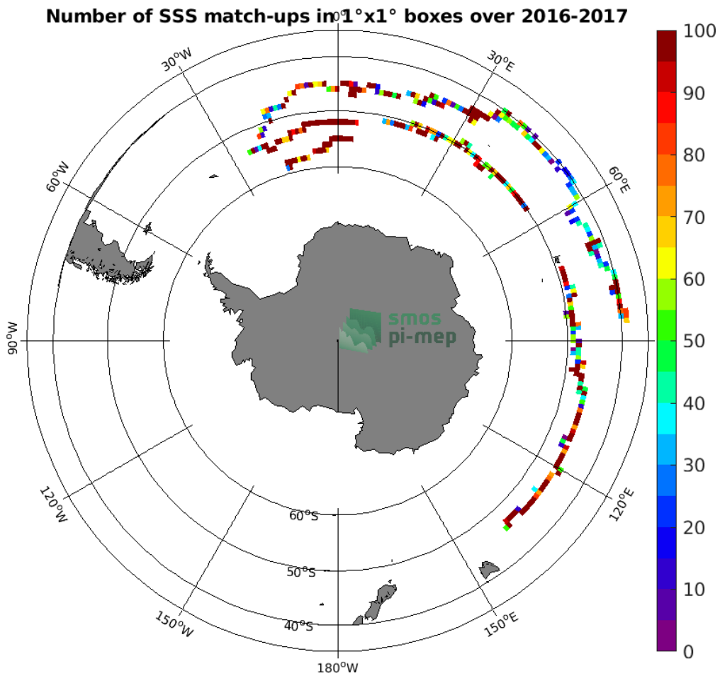
Figure 3: Number of SSS match-ups between Surface drifters SSS and the SMOS SSS L3 v2 - Daily - 0.5 Deg (CATDS-CECOS-IFREMER) SSS product for the Roaring Forties and Furious Fifties Pi-MEP region over 1^{\circ} \times 1^{\circ} boxes and for the full satellite product period.
