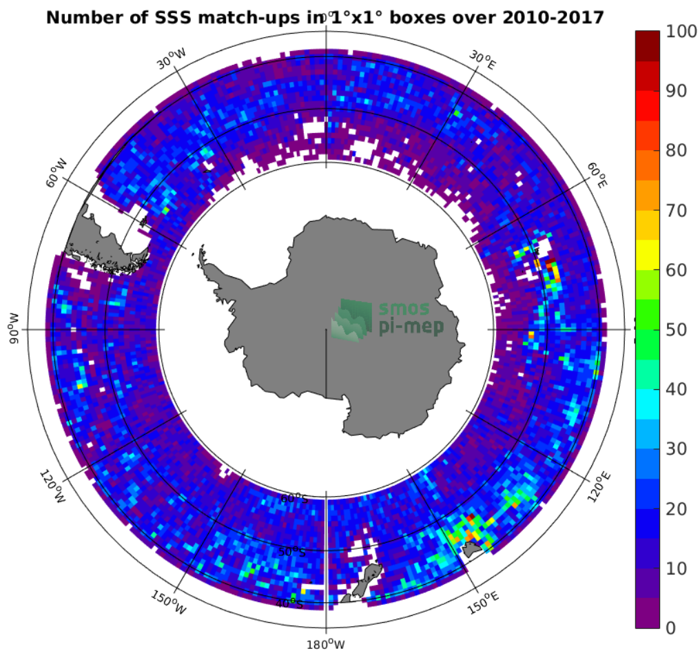
Figure 4: Number of SSS match-ups between Argo SSS and the SMOS-L3-CATDS-CECOS-IFREMER-V2-1DAY-0.5DEG SSS product for the Roaring Forties and Furious Fifties Pi-MEP region over 1^\circ \times 1^\circ boxes and for the full satellite product period.
