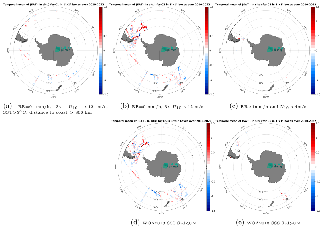
Figure 14: Temporal mean gridded over spatial boxes of size 1^\circ \times 1^\circ of \Delta\text{SSS} (SMOS SSS L3 v335 - Monthly - 25 km (CATDS-CPDC) - TSG (SAMOS)) for 5 different subdatasets corresponding to:RR=0 mm/h, 3 < U_{10} < 12 m/s, SST>5°C, distance to coast > 800 km (a), RR=0 mm/h, 3 < U_{10} < 12 m/s (b), RR>1mm/h and U_{10} < 4 m/s (c), WOA2013 SSS Std<0.2 (d), WOA2013 SSS Std>0.2 (e).
