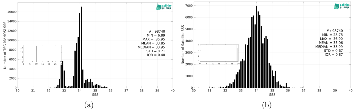
Figure 3: Histograms of SSS from TSG (SAMOS) (a) and SMOS SSS L3 v335 - Monthly - 25 km (CATDS-CPDC) (b) considering all match-up pairs per bins of 0.1 over the Roaring Forties and Furious Fifties Pi-MEP region and for the full satellite product period.
