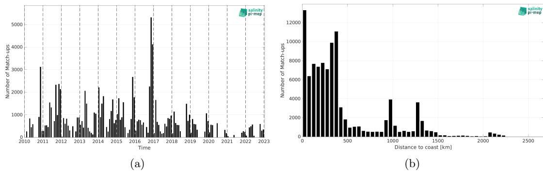
Figure 2: Number of match-ups between TSG (SAMOS) and SMOS SSS L3 v335 - Monthly - 25 km (CATDS-CPDC) SSS as a function of time (a) and as function of the distance to coast (b) over the Roaring Forties and Furious Fifties Pi-MEP region and for the full satellite product period.
