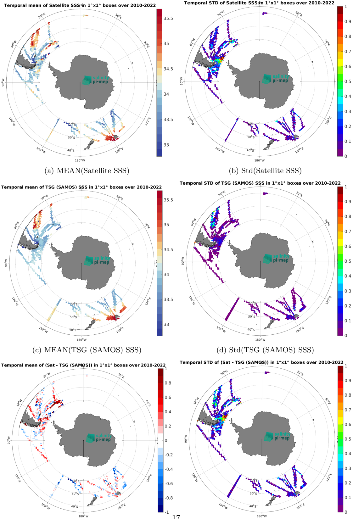
(e) MEAN( \Delta SSS) (Satellite - TSG (SAMOS))
