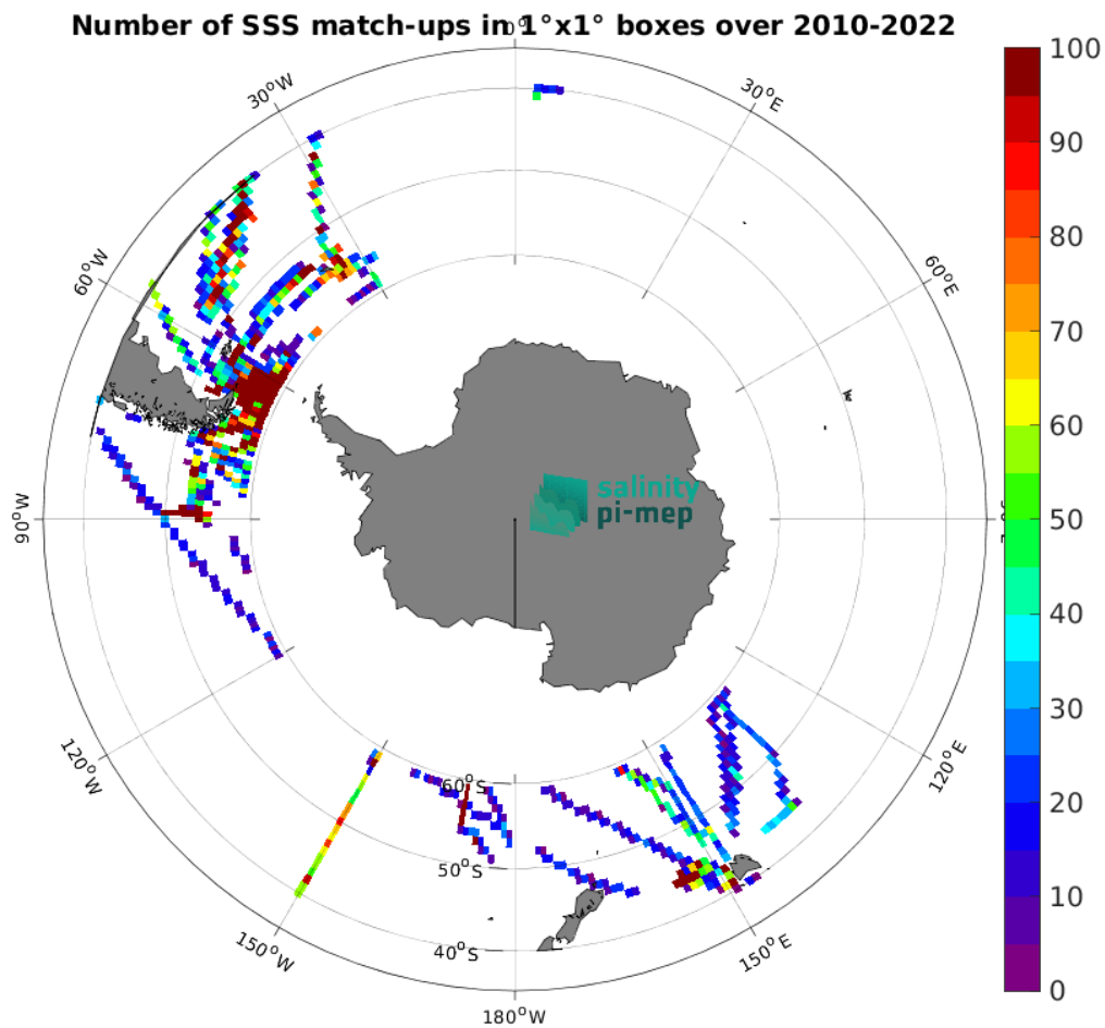
Figure 5: Number of SSS match-ups between TSG (SAMOS) SSS and the SMOS SSS L3 v335 - Monthly - 25 km (CATDS-CPDC) SSS product for the Roaring Forties and Furious Fifties Pi-MEP region over 1^\circ \times 1^\circ boxes and for the full satellite product period.
