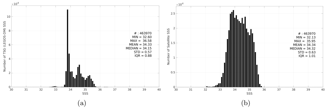
Figure 3: Histograms of SSS from TSG (LEGOS-DM) (a) and SMOS SSS L3 v335 - Monthly - 25 km (CATDS-CPDC) (b) considering all match-up pairs per bins of 0.1 over the Roaring Forties and Furious Fifties Pi-MEP region and for the full satellite product period.
