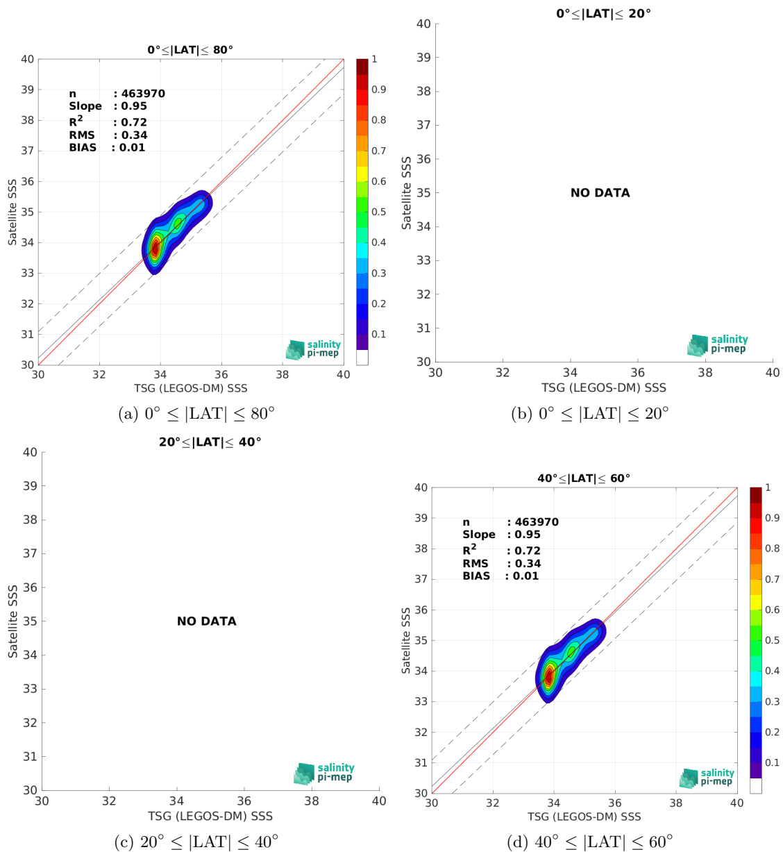
Figure 10: Contour maps of the concentration of SMOS SSS L3 v335 - Monthly - 25 km (CATDS-CPDC) SSS (y-axis) versus TSG (LEGOS-DM) SSS (x-axis) at match-up pairs for different latitude bands. For each plot, the red line shows x=y . The black thin and dashed lines indicate a linear fit through the data cloud and the \pm 95\% confidence levels, respectively. The number match-up pairs n , the slope and R^2 coefficient of the linear fit, the root mean square (RMS) and the mean bias between satellite and in situ data are indicated for each latitude band in each plots.
