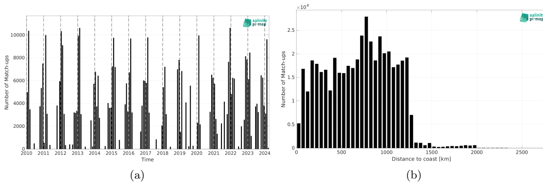
Figure 2: Number of match-ups between TSG (LEGOS-DM) and SMOS SSS L3 v335 - Monthly - 25 km (CATDS-CPDC) SSS as a function of time (a) and as function of the distance to coast (b) over the Roaring Forties and Furious Fifties Pi-MEP region and for the full satellite product period.
