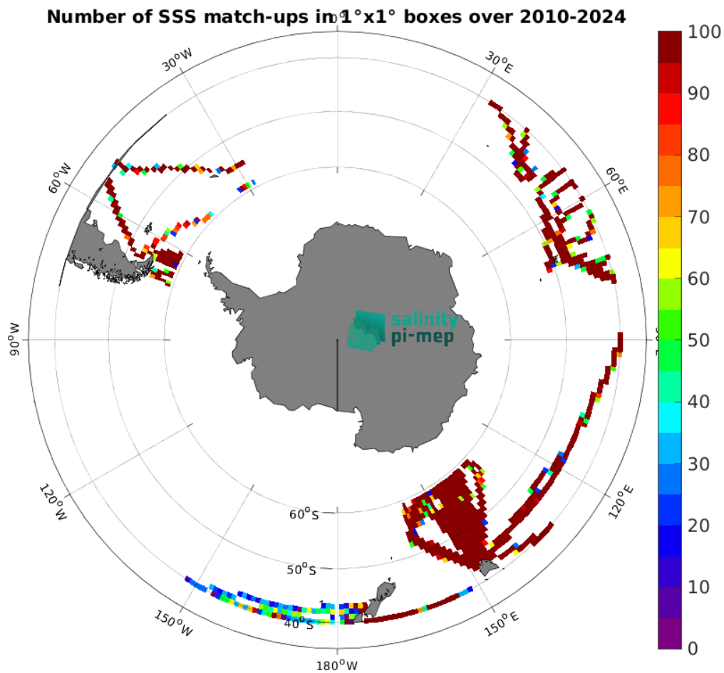
Figure 5: Number of SSS match-ups between TSG (LEGOS-DM) SSS and the SMOS SSS L3 v335 - Monthly - 25 km (CATDS-CPDC) SSS product for the Roaring Forties and Furious Fifties Pi-MEP region over 1^\circ \times 1^\circ boxes and for the full satellite product period.
