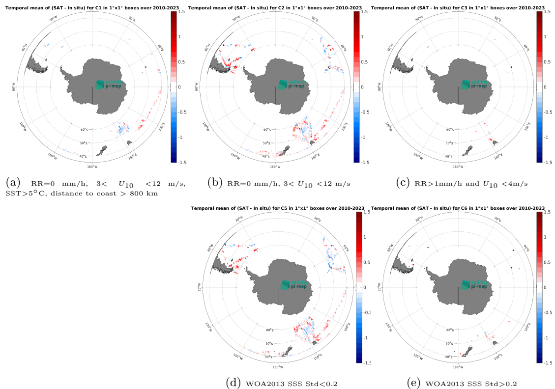
Figure 14: Temporal mean gridded over spatial boxes of size 1^\circ \times 1^\circ of \Delta\text{SSS} (SMOS SSS L3 v335 - Monthly - 25 km (CATDS-CPDC) - TSG (LEGOS-DM)) for 5 different subdatasets corresponding to:RR=0 mm/h, 3 < U_{10} < 12 m/s, SST>5°C, distance to coast > 800 km (a), RR=0 mm/h, 3 < U_{10} < 12 m/s (b), RR>1mm/h and U_{10} < 4 m/s (c), WOA2013 SSS Std<0.2 (d), WOA2013 SSS Std>0.2 (e).
