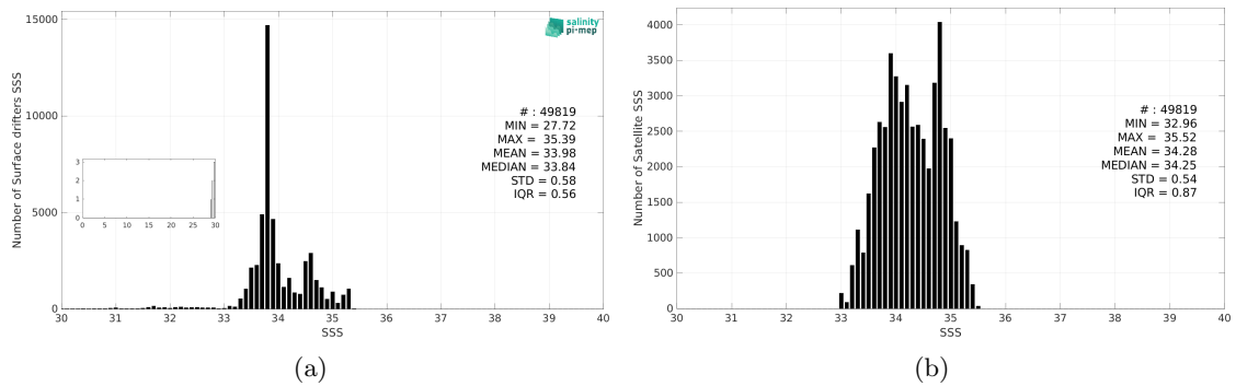
Figure 3: Histograms of SSS from Surface drifters (a) and SMOS SSS L3 v335 - Monthly - 25 km (CATDS-CPDC) (b) considering all match-up pairs per bins of 0.1 over the Roaring Forties and Furious Fifties Pi-MEP region and for the full satellite product period.
