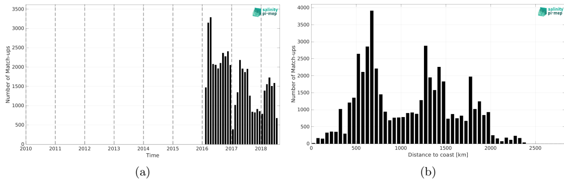
Figure 2: Number of match-ups between Surface drifters and SMOS SSS L3 v335 - Monthly - 25 km (CATDS-CPDC) SSS as a function of time (a) and as function of the distance to coast (b) over the Roaring Forties and Furious Fifties Pi-MEP region and for the full satellite product period.
