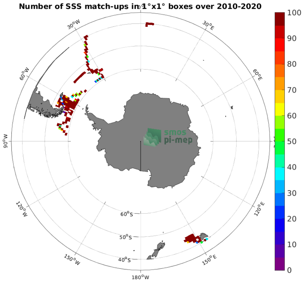
Figure 4: Number of SSS match-ups between TSG (SAMOS) SSS and the SMOS SSS L3 v335 - 10 Days - 25 km (CATDS-CPDC) SSS product for the Roaring Forties and Furious Fifties Pi-MEP region over 1^{\circ} \times 1^{\circ} boxes and for the full satellite product period.
