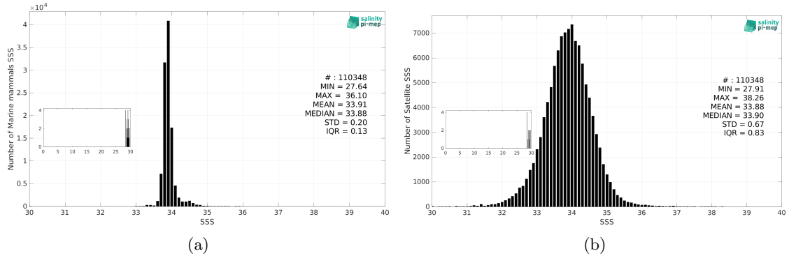
Figure 3: Histograms of SSS from Marine mammals (a) and SMOS SSS L3 v335 - 10 Days - 25 km (CATDS-CPDC) (b) considering all match-up pairs per bins of 0.1 over the Roaring Forties and Furious Fifties Pi-MEP region and for the full satellite product period.
