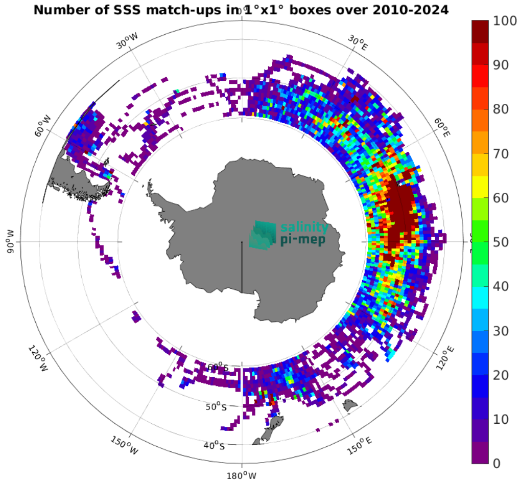
Figure 5: Number of SSS match-ups between Marine mammals SSS and the SMOS SSS L3 v335 - 10 Days - 25 km (CATDS-CPDC) SSS product for the Roaring Forties and Furious Fifties Pi-MEP region over 1^\circ \times 1^\circ boxes and for the full satellite product period.
