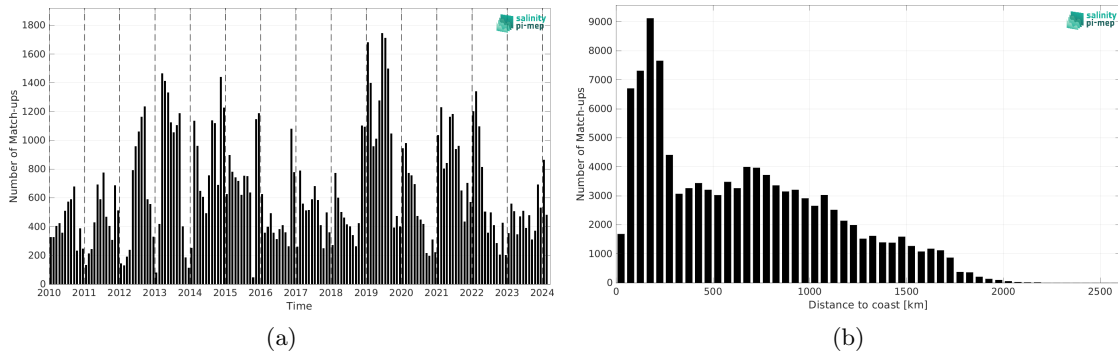
Figure 2: Number of match-ups between Marine mammals and SMOS SSS L3 v335 - 10 Days - 25 km (CATDS-CPDC) SSS as a function of time (a) and as function of the distance to coast (b) over the Roaring Forties and Furious Fifties Pi-MEP region and for the full satellite product period.
