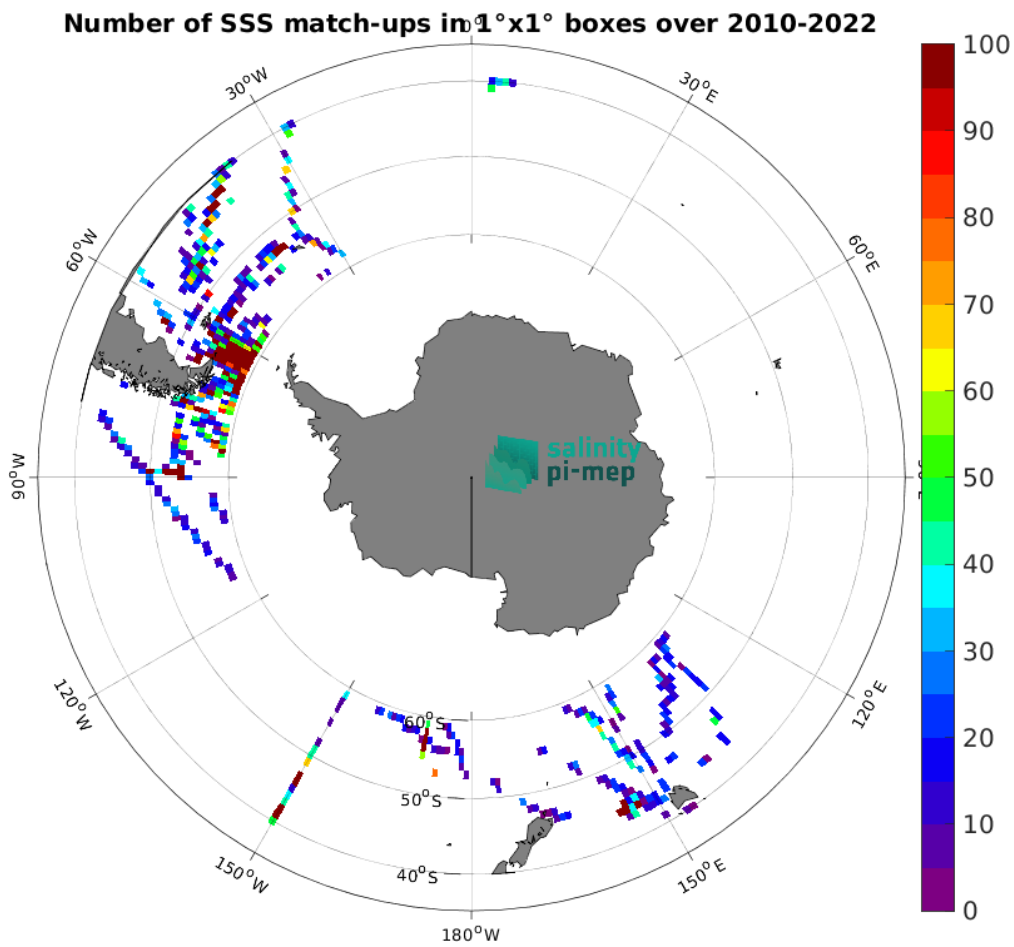
Figure 5: Number of SSS match-ups between TSG (SAMOS) SSS and the SMOS SSS L2Q v333 - 0.25 Deg (CATDS-CPDC) SSS product for the Roaring Forties and Furious Fifties Pi-MEP region over 1^\circ \times 1^\circ boxes and for the full satellite product period.
