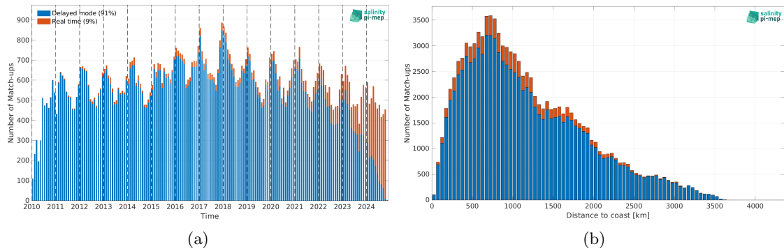
Figure 2: Number of match-ups between Argo and SMOS SSS L2Q v333 - 0.25 Deg (CATDS-CPDC) SSS as a function of time (a) and as function of the distance to coast (b) over the Roaring Forties and Furious Fifties Pi-MEP region and for the full satellite product period.
