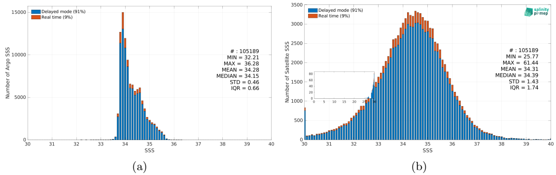
Figure 3: Histograms of SSS from Argo (a) and SMOS SSS L2Q v333 - 0.25 Deg (CATDS-CPDC) (b) considering all match-up pairs per bins of 0.1 over the Roaring Forties and Furious Fifties Pi-MEP region and for the full satellite product period.
