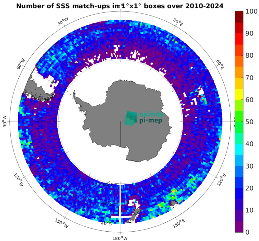
Figure 5: Number of SSS match-ups between Argo SSS and the SMOS SSS L2Q v333 - 0.25 Deg (CATDS-CPDC) SSS product for the Roaring Forties and Furious Fifties Pi-MEP region over 1^\circ \times 1^\circ boxes and for the full satellite product period.
