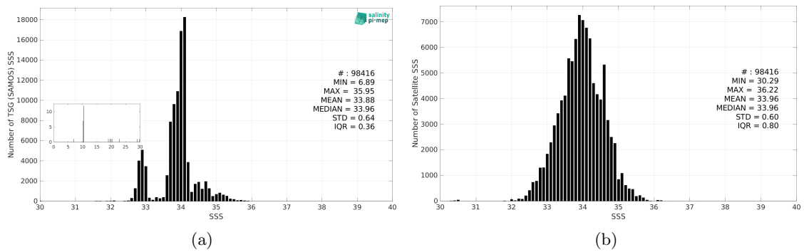
Figure 3: Histograms of SSS from TSG (SAMOS) (a) and SMOS SSS L3 v332 - 9 Days (CATDS-CPDC) (b) considering all match-up pairs per bins of 0.1 over the Roaring Forties and Furious Fifties Pi-MEP region and for the full satellite product period.
