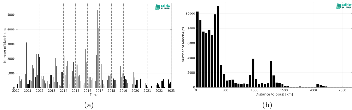
Figure 2: Number of match-ups between TSG (SAMOS) and SMOS SSS L3 v332 - 9 Days (CATDS-CPDC) SSS as a function of time (a) and as function of the distance to coast (b) over the Roaring Forties and Furious Fifties Pi-MEP region and for the full satellite product period.
