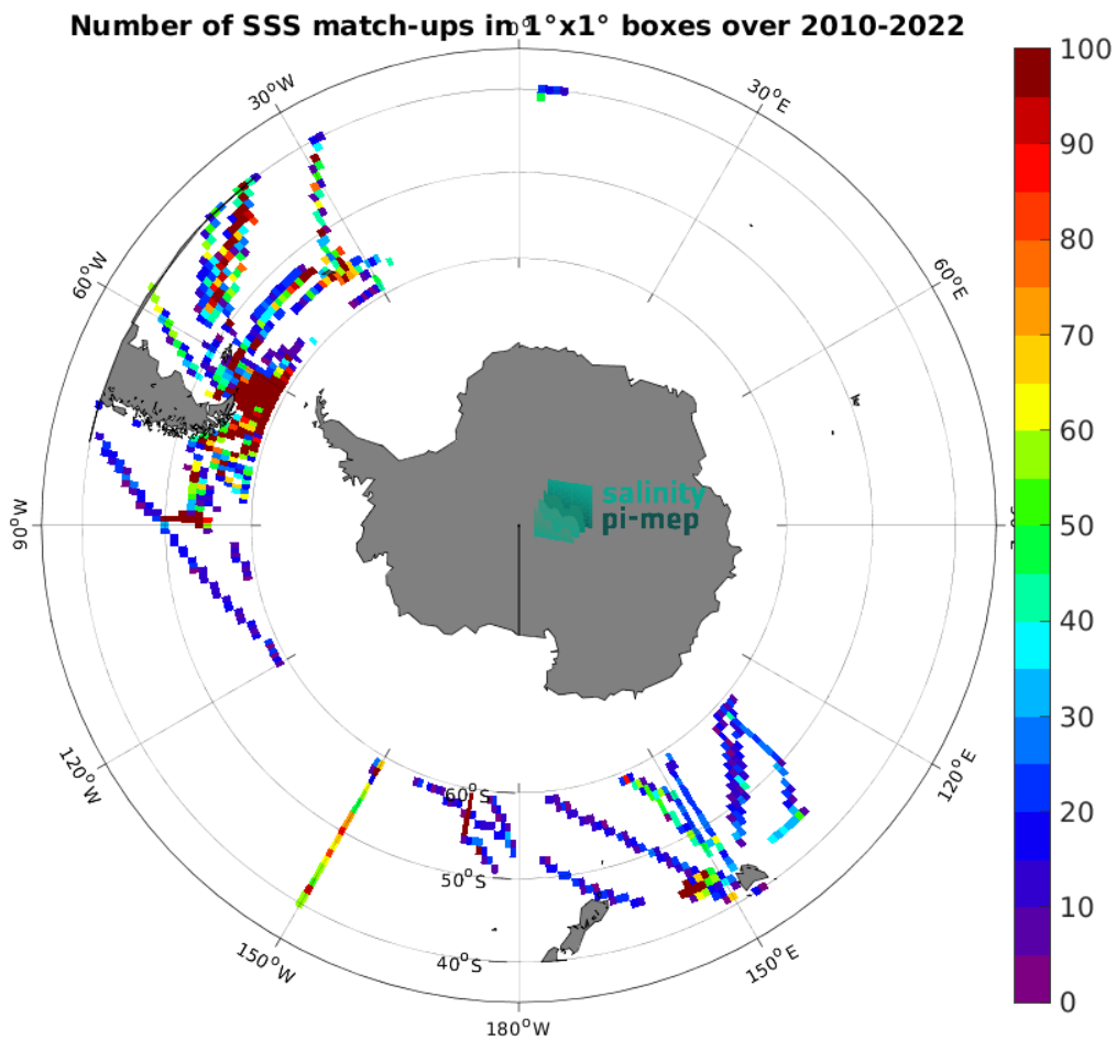
Figure 5: Number of SSS match-ups between TSG (SAMOS) SSS and the SMOS SSS L3 v332 - 9 Days (CATDS-CPDC) SSS product for the Roaring Forties and Furious Fifties Pi-MEP region over 1^\circ \times 1^\circ boxes and for the full satellite product period.
