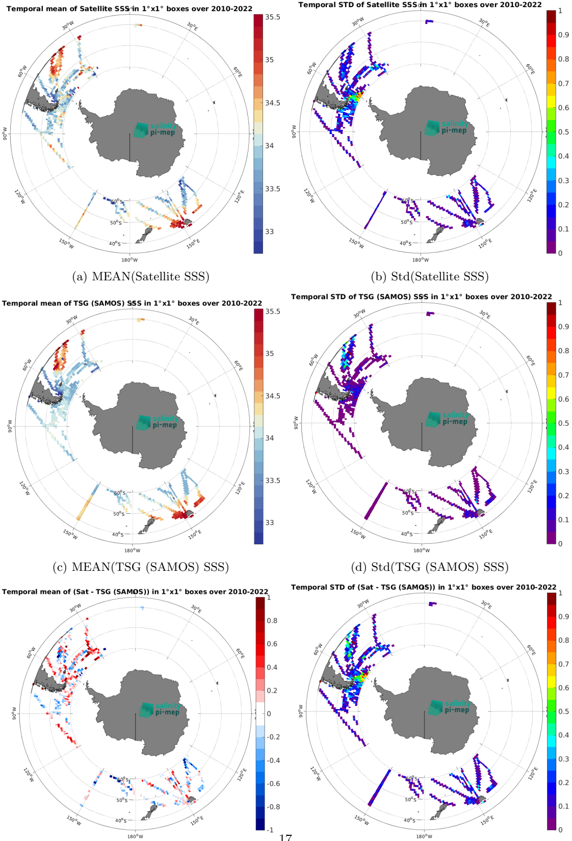
(e) MEAN( \Delta SSS) (Satellite - TSG (SAMOS)) (f) Std( \Delta SSS) (Satellite - TSG (SAMOS)) Figure 7: Temporal mean (left) and Std (right) of SSS from SMOS SSS L3 v332 - 9 Days (CATDS-CPDC) (top), TSG (SAMOS) (middle), and of \Delta SSS (Satellite - TSG (SAMOS)). Only match-up pairs are used to generate these maps.
