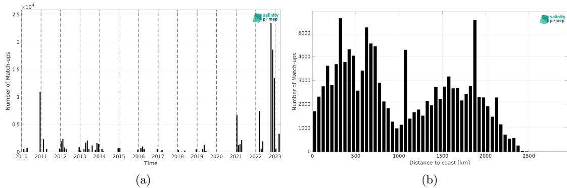
Figure 2: Number of match-ups between TSG (Polarstern) and SMOS SSS L3 v332 - 9 Days (CATDS-CPDC) SSS as a function of time (a) and as function of the distance to coast (b) over the Roaring Forties and Furious Fifties Pi-MEP region and for the full satellite product period.
