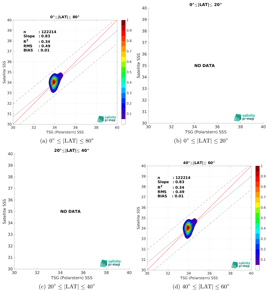
Figure 10: Contour maps of the concentration of SMOS SSS L3 v332 - 9 Days (CATDS-CPDC) SSS (y-axis) versus TSG (Polarstern) SSS (x-axis) at match-up pairs for different latitude bands. For each plot, the red line shows x=y . The black thin and dashed lines indicate a linear fit through the data cloud and the \pm 95\% confidence levels, respectively. The number match-up pairs n , the slope and R^2 coefficient of the linear fit, the root mean square (RMS) and the mean bias between satellite and in situ data are indicated for each latitude band in each plot.
