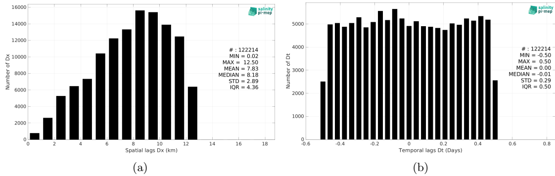
Figure 6: Histograms of the spatial (a) and temporal (b) lags between the location/time of the TSG (Polarstern) measurement and the date of the corresponding SMOS SSS L3 v332 - 9 Days (CATDS-CPDC) SSS pixel.
