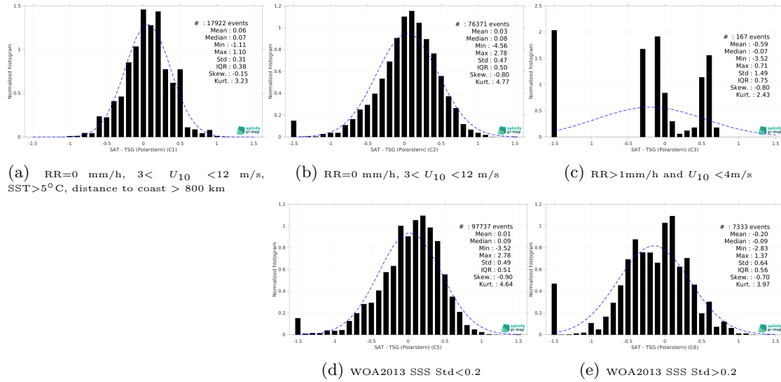
Figure 15: Normalized histogram of \Delta SSS (SMOS SSS L3 v332 - 9 Days (CATDS-CPDC) - TSG (Polarstern)) for 5 different subdatasets corresponding to: RR=0 mm/h, 3 < U_{10} < 12 m/s, SST > 5°C, distance to coast > 800 km (a), RR=0 mm/h, 3 < U_{10} < 12 m/s (b), RR > 1mm/h and U_{10} < 4 m/s (c), WOA2013 SSS Std < 0.2 (d), WOA2013 SSS Std > 0.2 (e).
