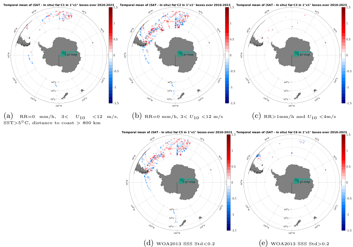
Figure 14: Temporal mean gridded over spatial boxes of size 1^\circ \times 1^\circ of \Delta SSS (SMOS SSS L3 v332 - 9 Days (CATDS-CPDC) - TSG (Polarstern)) for 5 different subdatasets corresponding to:RR=0 mm/h, 3 < U_{10} < 12 m/s, SST >5^\circ C, distance to coast > 800 km (a), RR=0 mm/h, 3 < U_{10} < 12 m/s (b), RR >1 mm/h and U_{10} < 4 m/s (c), WOA2013 SSS Std <0.2 (d), WOA2013 SSS Std >0.2 (e).
