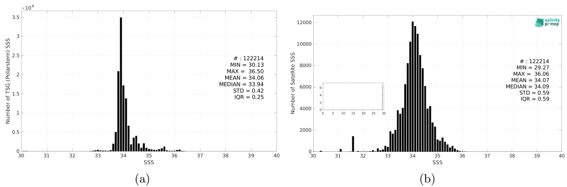
Figure 3: Histograms of SSS from TSG (Polarstern) (a) and SMOS SSS L3 v332 - 9 Days (CATDS-CPDC) (b) considering all match-up pairs per bins of 0.1 over the Roaring Forties and Furious Fifties Pi-MEP region and for the full satellite product period.
