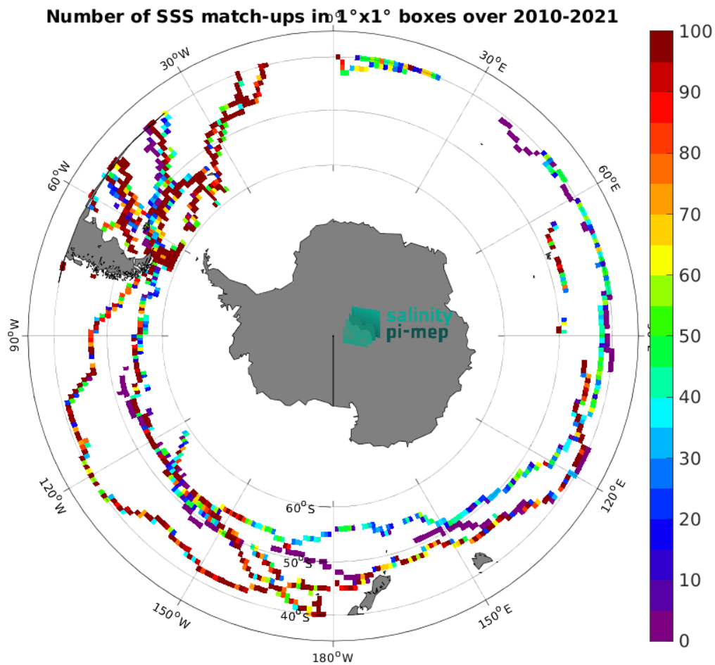
Figure 5: Number of SSS match-ups between TSG (GOSUD-Sailing-ship) SSS and the SMOS SSS L3 v332 - 9 Days (CATDS-CPDC) SSS product for the Roaring Forties and Furious Fifties Pi-MEP region over 1^{\circ} \times 1^{\circ} boxes and for the full satellite product period.
