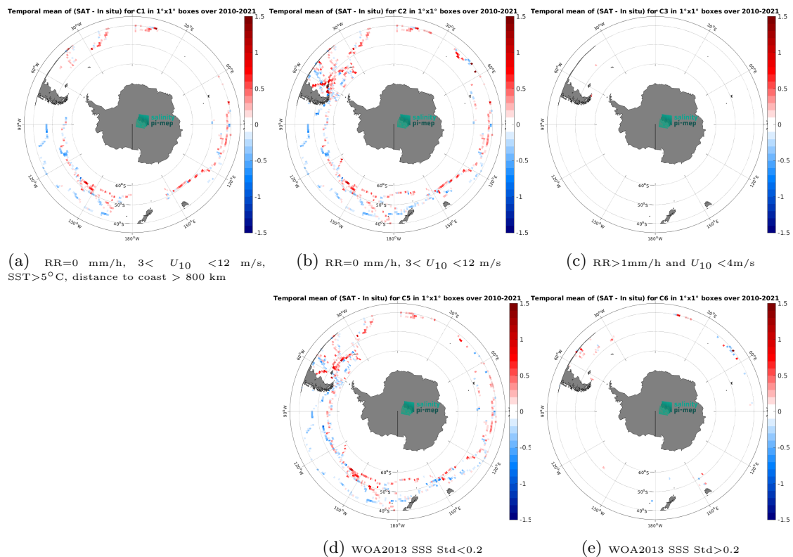
Figure 14: Temporal mean gridded over spatial boxes of size 1^\circ \times 1^\circ of \Delta\text{SSS} (SMOS SSS L3 v332 - 9 Days (CATDS-CPDC) - TSG (GOSUD-Sailing-ship)) for 5 different subdatasets corresponding to:RR=0 mm/h, 3 < U_{10} < 12 m/s, SST >5^\circ\text{C} , distance to coast > 800 km (a), RR=0 mm/h, 3 < U_{10} < 12 m/s (b), RR >1 mm/h and U_{10} < 4 m/s (c), WOA2013 SSS Std <0.2 (d), WOA2013 SSS Std >0.2 (e).
