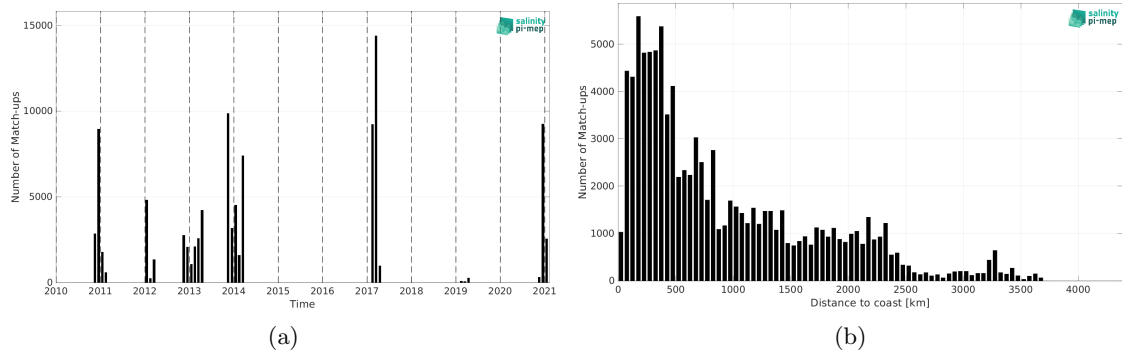
Figure 2: Number of match-ups between TSG (GOSUD-Sailing-ship) and SMOS SSS L3 v332 - 9 Days (CATDS-CPDC) SSS as a function of time (a) and as function of the distance to coast (b) over the Roaring Forties and Furious Fifties Pi-MEP region and for the full satellite product period.
