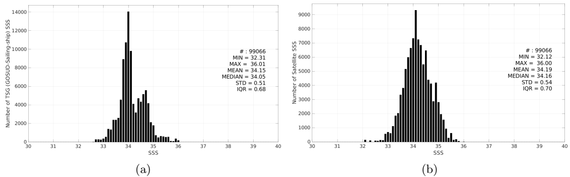
Figure 3: Histograms of SSS from TSG (GOSUD-Sailing-ship) (a) and SMOS SSS L3 v332 - 9 Days (CATDS-CPDC) (b) considering all match-up pairs per bins of 0.1 over the Roaring Forties and Furious Fifties Pi-MEP region and for the full satellite product period.
