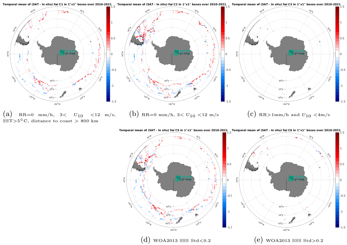
Figure 12: Temporal mean gridded over spatial boxes of size 1°×1° of \Delta SSS (SMOS SSS L3 v332 - 9 Days (CATDS-CPDC) - TSG (GOSUD-Sailing-ship)) for 5 different subdatasets corresponding to: RR=0 mm/h, 3 < U_{10} < 12 m/s, SST>5°C, distance to coast > 800 km (a), RR=0 mm/h, 3 < U_{10} < 12 m/s (b), RR>1mm/h and U_{10} < 4 m/s (c), WOA2013 SSS Std<0.2 (d), WOA2013 SSS Std>0.2 (e).
