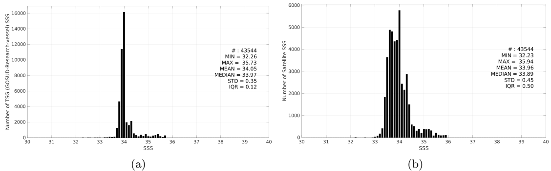
Figure 3: Histograms of SSS from TSG (GOSUD-Research-vessel) (a) and SMOS SSS L3 v332 - 9 Days (CATDS-CPDC) (b) considering all match-up pairs per bins of 0.1 over the Roaring Forties and Furious Fifties Pi-MEP region and for the full satellite product period.
