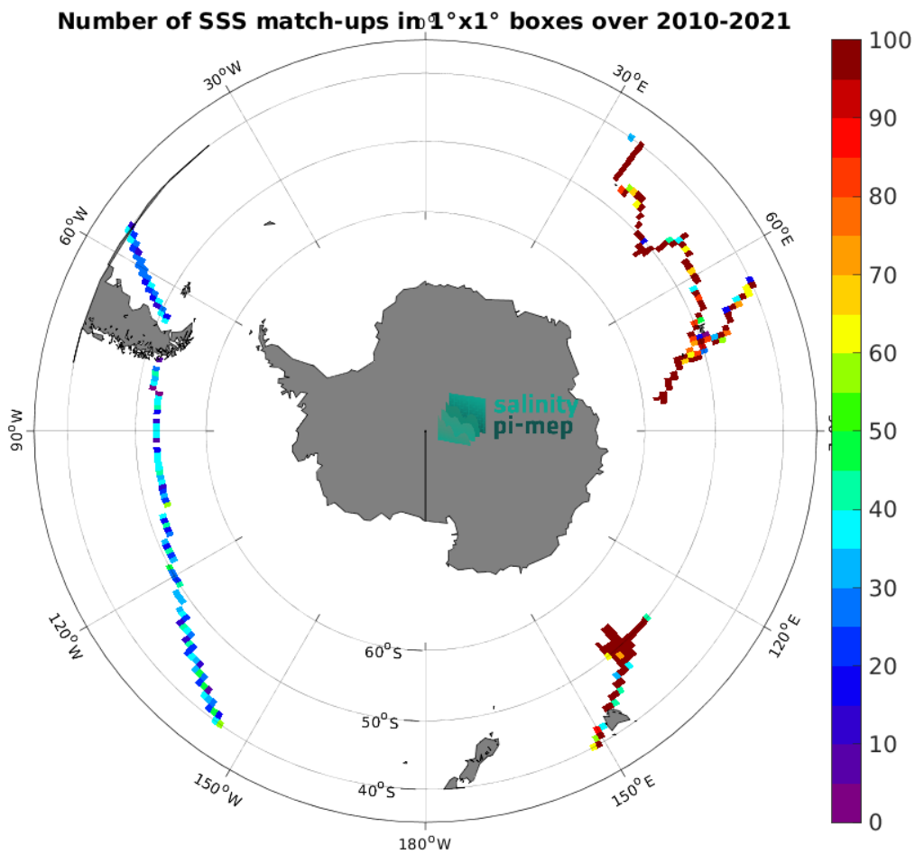
Figure 5: Number of SSS match-ups between TSG (GOSUD-Research-vessel) SSS and the SMOS SSS L3 v332 - 9 Days (CATDS-CPDC) SSS product for the Roaring Forties and Furious Fifties Pi-MEP region over 1^\circ \times 1^\circ boxes and for the full satellite product period.
