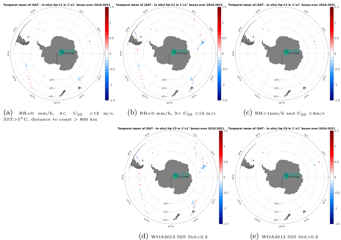
Figure 14: Temporal mean gridded over spatial boxes of size 1^\circ \times 1^\circ of \Delta SSS (SMOS SSS L3 v332 - 9 Days (CATDS-CPDC) - TSG (GOSUD-Research-vessel)) for 5 different subdatasets corresponding to:RR=0 mm/h, 3 < U_{10} < 12 m/s, SST > 5^\circ\text{C} , distance to coast > 800 km (a), RR=0 mm/h, 3 < U_{10} < 12 m/s (b), RR > 1 mm/h and U_{10} < 4 m/s (c), WOA2013 SSS Std < 0.2 (d), WOA2013 SSS Std > 0.2 (e).
