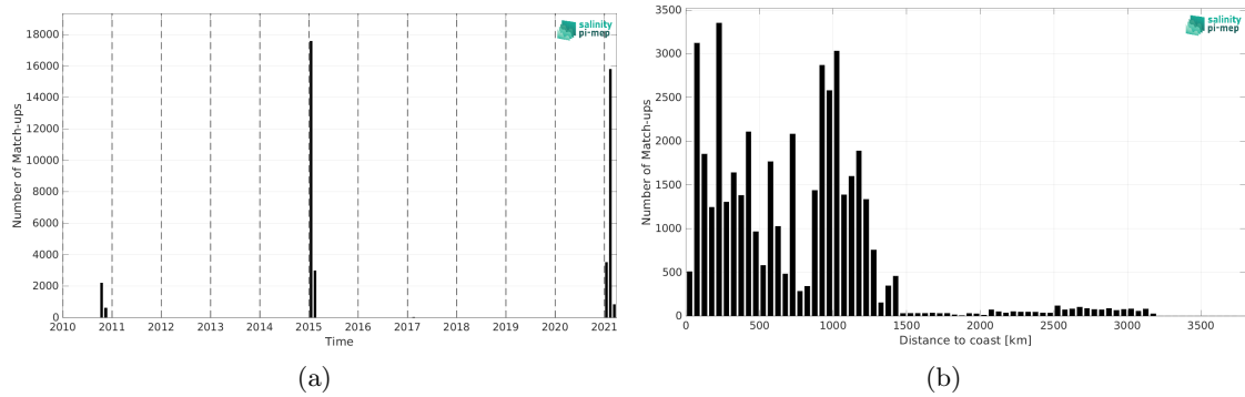
Figure 2: Number of match-ups between TSG (GOSUD-Research-vessel) and SMOS SSS L3 v332 - 9 Days (CATDS-CPDC) SSS as a function of time (a) and as function of the distance to coast (b) over the Roaring Forties and Furious Fifties Pi-MEP region and for the full satellite product period.
