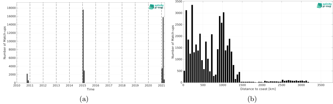
Figure 1: Number of match-ups between TSG (GOSUD-Research-vessel) and SMOS SSS L3 v332 - 9 Days (CATDS-CPDC) SSS as a function of time (a) and as function of the distance to coast (b) over the Roaring Forties and Furious Fifties Pi-MEP region and for the full satellite product period.
