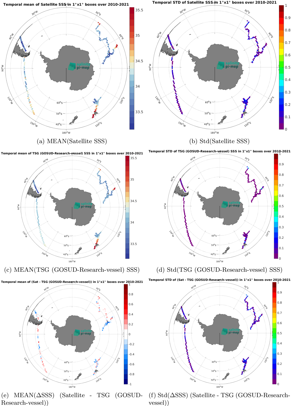
Figure 6: Temporal mean (left) and Std (right) of SSS from SMOS SSS L3 v332 - 9 Days (CATDS-CPDC) (top), TSG (GOSUD-Research-vessel) (middle), and of \Delta SSS (Satellite - TSG (GOSUD-Research-vessel)). Only match-up pairs are used to generate these maps.
