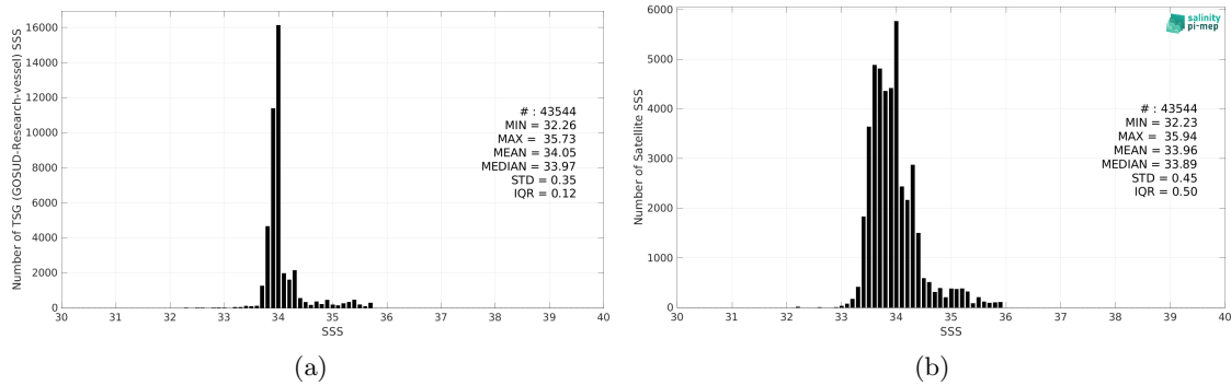
Figure 2: Histograms of SSS from TSG (GOSUD-Research-vessel) (a) and SMOS SSS L3 v332 - 9 Days (CATDS-CPDC) (b) considering all match-up pairs per bins of 0.1 over the Roaring Forties and Furious Fifties Pi-MEP region and for the full satellite product period.
