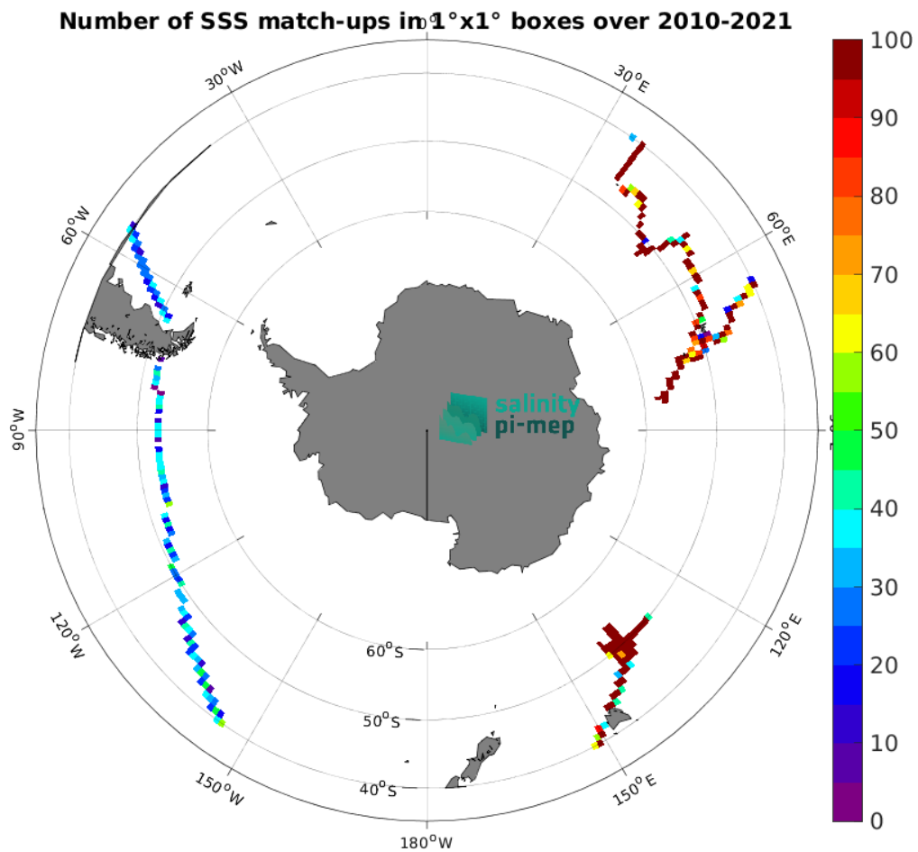
Figure 4: Number of SSS match-ups between TSG (GOSUD-Research-vessel) SSS and the SMOS SSS L3 v332 - 9 Days (CATDS-CPDC) SSS product for the Roaring Forties and Furious Fifties Pi-MEP region over 1^{\circ} \times 1^{\circ} boxes and for the full satellite product period.
